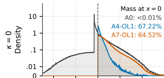
FFN activations
