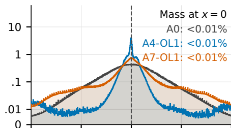
Attention activations
