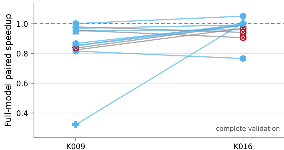
70M: generic K009 → topology-specific K016
