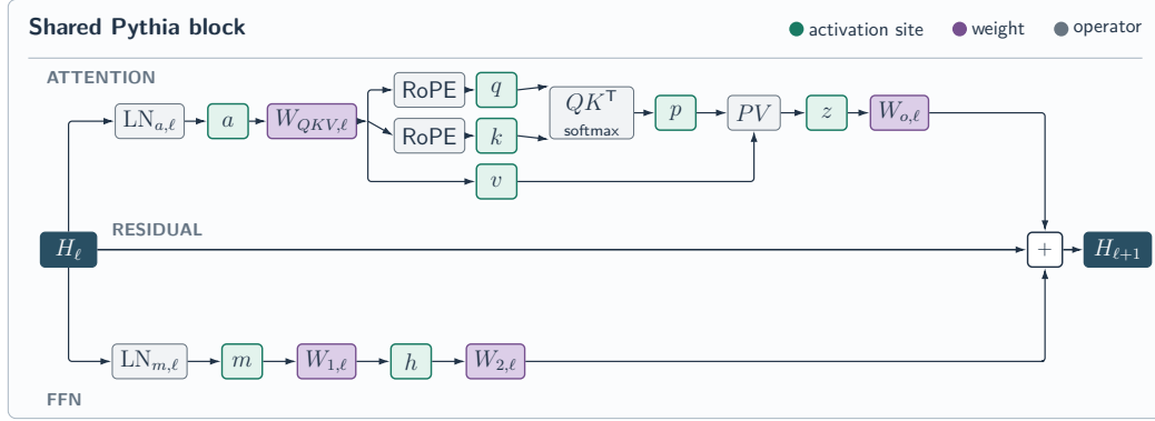
Figure 1: Activation sites in the shared Pythia block. A1-H replaces GELU at h with ReLU. A4 applies G_{\pm, \kappa} at a, m, h, z ; A7 adds G_{\pm, \kappa} at post-RoPE q, k and at v . Pressure variants target every selected site. A0 retains GELU. Appendix C.1 gives the full recipe diagram and tensor shapes.
