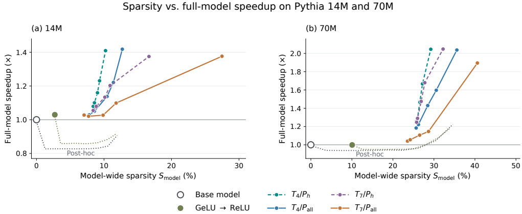
Figure 3: From model-wide sparsity to measured speedup. Pythia-14M (a) and 70M (b), with 22 trained checkpoints and 20 post-hoc clipping settings per size. Speedup divides the same-size base-model latency by each setting’s latency, using the final specialized implementation for both terms; it is not speedup over native execution. Dashed/solid curves connect h-only/all-site pressure settings; dotted paths show base/ReLU clipping, including its recurring cost. Timings use RTX5090, BF16, batch one, 2,048 tokens and the full logit head. Sparsity uses full-validation pooled logical counts. Panel scales differ; normalization does not remove differences in model quality or timing sessions.
