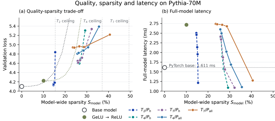
Figure 4: Quality, sparsity and execution on Pythia-70M. (a) Validation loss and (b) full-model latency versus S_{\text{model}} for 27 checkpoints: Base, GeLU \rightarrow ReLU, T_2/P_h , and T_4/T_7 with P_h or P_{\text{all}} , each thresholded recipe at \kappa = 0, .01, .05, .1, .5 . Colors and line styles match Figure ???. Dotted curves in (a) apply post-hoc clipping to the fixed Base/ReLU controls; high-loss tails extend beyond the view. Vertical guides mark sparsity ceilings. In (b), the Base marker and horizontal reference use native PyTorch/SDPA (1.611 ms); all other markers use the optimized 70M kernel. Measurements use RTX 5090 GPUs, three fresh processes per checkpoint, batch one, 2,048 tokens and full output logits. Appendix E.4 compares the native, original-port and optimized implementations and reports the timing references.
