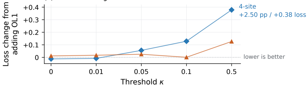
(a) Effect of adding OL1 on validation loss
