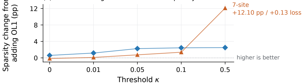
(b) Effect of adding OL1 on model-wide sparsity
