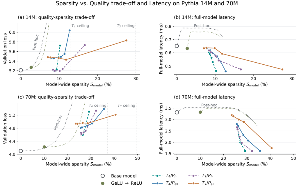
Figure 1: Quality and execution depend on threshold and pressure placement. Rows show Pythia-14M (a,b) and 70M (c,d); columns show final validation loss and full-model latency versus \mathcal{S}_{\text{model}} . Each row contains 22 checkpoints: the Base Model ( T_0/P_0 ), GeLU \rightarrow ReLU at h ( T_1/P_0 ), and T_4/T_7 thresholding at four/seven sites with OL1 pressure at h ( P_h , dashed) or all thresholded sites ( P_{all} , solid). Pressure curves connect separate \kappa \in \{0, .01, .05, .1, .5\} runs, each with one seed and one final checkpoint. Dotted post-hoc paths clip the fixed controls at a, m, h, z for p = 0, .1, \dots, .9 . All 40 clipping latencies are measured, including recurring clipping operators at positive targets. Eight 14M and seven 70M high-loss clipping points lie above the quality views (full paths in Figures 12 and 13). Vertical guides mark analytic sparsity ceilings. Loss and count-pooled sparsity use FP16 validation over all 338 complete blocks from 500 documents, excluding the 1,444-token tail. Latencies use K050 at 14M and its qualified 70M port: RTX5090, BF16, batch one, 2,048-token uncached inference, all 50,304 logits, and a geometric mean over 1,344 host timings per setting. Timing sessions differ across cohorts; small cross-session differences are descriptive. Axes have independent ranges between model sizes.
