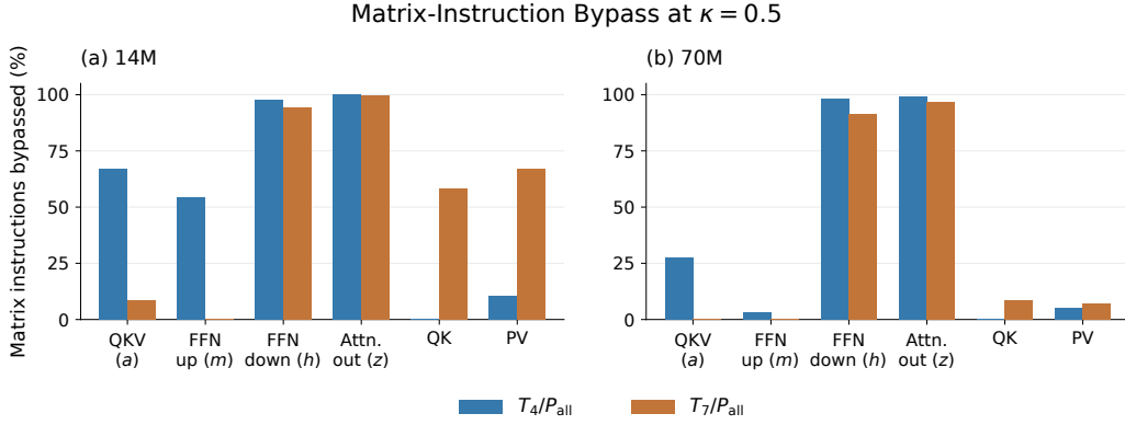
Figure 6: Skippable work is not the same as saved time. Matrix instructions bypassed for T_4/P_{all} and T_7/P_{all} at \kappa = 0.5 : (a) 14M and (b) 70M. Each bar pools bypassed instructions divided by issued plus bypassed instructions over all layers and complete validation. Labels identify each operation and its input site. Bypass at h/z includes replacement by a few scalar operations; attention counts include causal masking and padding. The bars do not measure latency or the fraction of total model work saved.
