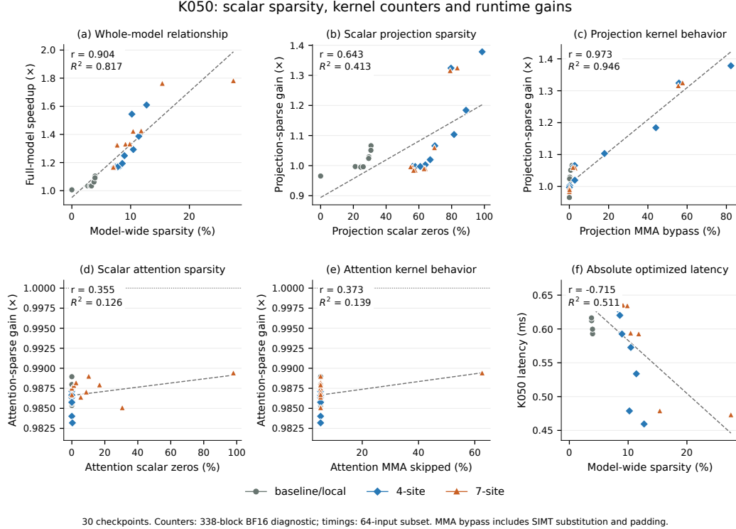
Figure 17: Scalar sparsity, skipped instructions, and matched runtime gains. The 30 checkpoints share colors and shapes by family. Projection and attention gains are t_0/t_P and t_P/t_K ; lines are descriptive OLS fits with intercepts. Projection bypass includes scalar substitution and padded MMA rows. Attention skip fractions include masked/padded work and take only two distinct values. The remaining pages of the accompanying diagnostic PDF show within-family fits, matched threshold comparisons, and absolute latency traces. Counters cover 338 validation blocks, while timings cover 64 matched inputs.
