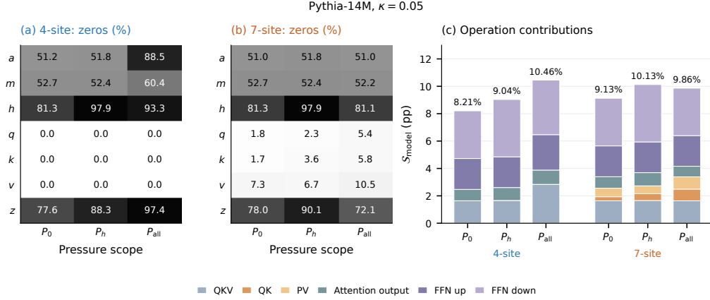
Figure 8: Pressure-scope effects at the moderate threshold \kappa = 0.05 . The six 14M recipes use the same count pooling and operation denominator as Figure 5. H-only pressure concentrates zeros at h while preserving a different pattern at m and Q/K/V from broad pressure. Rounded percentages do not establish all-zero or fully dense tensors.
