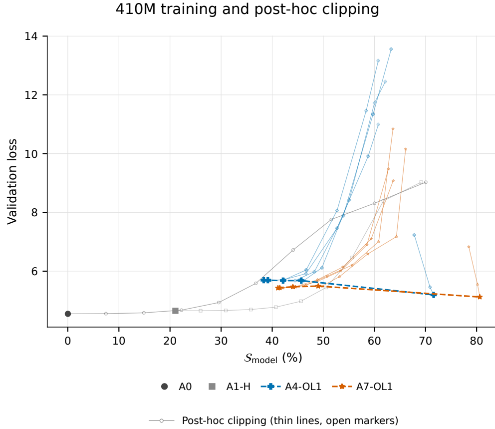
Figure 14: Complete 410M training and post-hoc thresholding results: 12 trained endpoints and 120 post-hoc thresholding evaluations. Large filled markers and bold lines identify the trained recipes; faint open-marker paths follow each checkpoint through ten increasing thresholding targets. All points, including overlaps and high-loss settings, are retained. The evaluation and line conventions match Figure 12.
