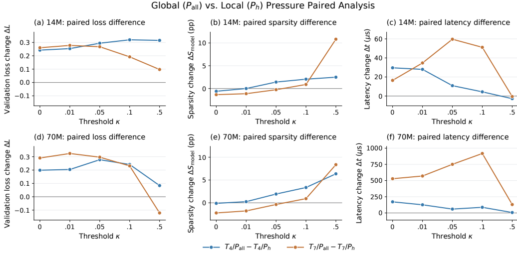
Figure 4: Paired effects of broadening pressure from P_h to P_{all} . Every point is all-site minus h-only pressure at matched model size, threshold scope and \kappa , with \lambda = b = 1 . Rows show 14M/70M; columns show loss change, sparsity change (pp), and full-model latency change ( \mu s ). Positive loss or latency differences favor P_h ; positive sparsity differences favor P_{all} . Latencies subtract checkpoint geometric means: RTX5090, BF16, batch one, 2,048 tokens, full logit head and 1,344 timings per checkpoint. The 14M T_7 pairs span GPU sessions; 70M uses the qualified K050 port. Small timing differences are descriptive. Lines connect separate single-seed runs with matched initialization, data order and training budget.
