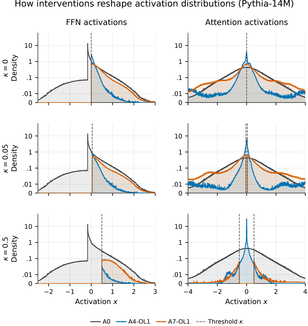
Figure 5: Interventions reshape FFN and attention distributions differently. Exact zeros are omitted from the curves and reported in Table 9. Columns pool FFN ( h, m ) and attention ( q, k, v ) activations; rows use trained thresholds \kappa = 0, 0.05, 0.5 . A0 is repeated across rows. Counts are pooled across all layers and validation blocks, weighting h : m by 80:20 and q : k : v equally. Density divides nonzero bin counts by all captured elements and bin width, without renormalizing the visible range. The vertical scale is symlog, linear below 0.01; filled areas on this scale do not represent probability mass. Dashed lines mark +\kappa for A4/A7 FFN thresholds and \pm\kappa for A7 attention thresholds. Q/K are measured after RoPE. A4 leaves q, k, v without direct thresholding or pressure; A7 targets them directly. The seven checkpoints use no additional post-hoc clipping.
