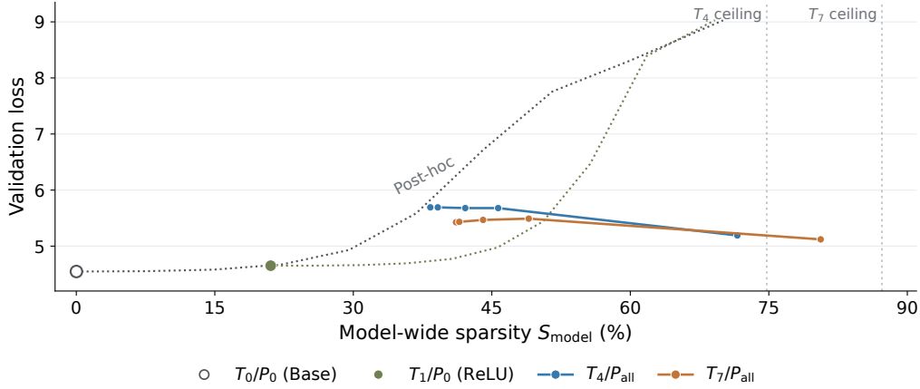
Figure 15: Complete 410M quality–sparsity stress-test panel. All twelve trained conditions: Base, ReLU, and T_4/P_{\text{all}} and T_7/P_{\text{all}} at \kappa = 0, .01, .05, .1, .5 . Dotted paths retain all ten post-hoc targets for each fixed Base/ReLU control, including their full loss range. Vertical guides mark the four- and seven-site sparsity ceilings. Trained losses use ordinary final-checkpoint validation; clipping retains its original FP16 pass. Sparsity pools logical counts over all 338 complete validation blocks. Figure 16 additionally retains the historical clipping sweeps of every trained recipe.
