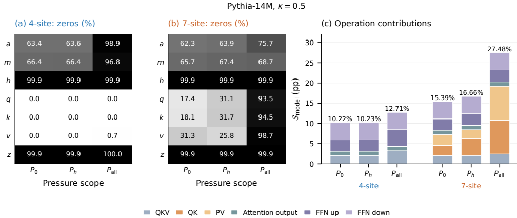
Figure 6: Pressure placement changes activation structure and its computational effect. All six multisite recipes at \kappa = 0.5 , Pythia-14M. (a,b) Exact-zero percentages at each site, pooled from integer counts across validation and layers; m and h are separate. P_{\text{all}} means P_4 or P_7 . Rounded 0.0/100.0 entries need not be exact endpoints. (c) Operation contributions use the common full-model product denominator; totals appear above each bar. Broad four-site pressure mainly increases projection-side opportunity, whereas broad seven-site pressure exposes large QK/PV contributions. These are logical zero-operand products, not measured runtime savings.
