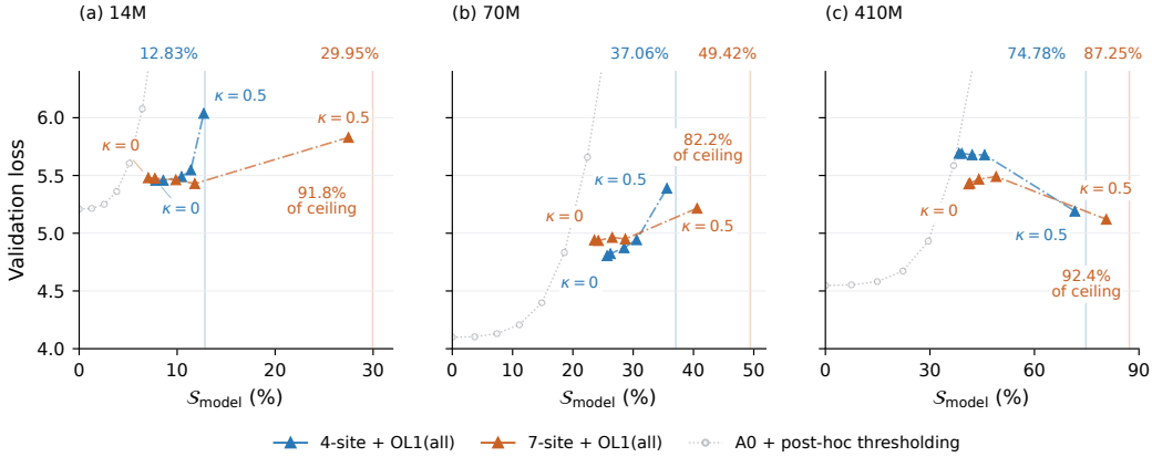
Figure 7: The high-threshold seven-site recipe remains better on both quality and model-wide sparsity across model sizes. Absolute validation loss versus model-wide sparsity S_{\text{model}} for Pythia-14M, 70M, and 410M. Blue and orange curves connect separately trained four-site + OL1(all) and seven-site + OL1(all) checkpoints at \kappa \in \{0, 0.01, 0.05, 0.1, 0.5\} ; the gray dotted curves apply post-hoc thresholding at a, m, h, z to the corresponding A0 checkpoints. Vertical guides mark the analytic four-site and seven-site sparsity ceilings, and annotations at the seven-site \kappa = 0.5 endpoints report the fraction of the seven-site ceiling reached. At \kappa = 0.5 , seven-site + OL1(all) has both lower validation loss and greater S_{\text{model}} than four-site + OL1(all) at all three sizes, reaching 91.8%, 82.2%, and 92.4% of the respective seven-site ceilings. The ordering at \kappa = 0 changes with size. Lines connect evaluated settings rather than interpolated models; full post-hoc thresholding trajectories, including higher-loss evaluations outside the displayed range, are reported in Appendix D.3.
