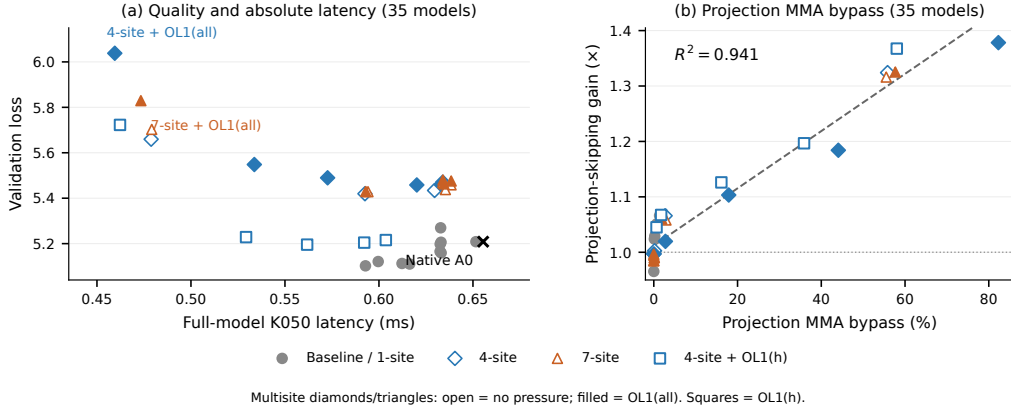
Figure 8: The runtime value of zeros depends on their execution structure. (a) Validation loss versus absolute full-model K050 latency for 35 qualified checkpoints; the black cross is native A0. Gray circles show A0 and one-site conditions, blue diamonds four-site recipes, and orange triangles seven-site recipes. These multisite markers are open without pressure and filled with OL1(all); blue squares add four-site OL1(h). This historical panel excludes the seven-site OL1(h) timings shown in Figure 1. (b) Projection MMA bypass for the same 35 checkpoints versus matched gain from enabling projection skipping: all-skips-off latency divided by projection-enabled, attention-dense latency. The dashed OLS fit is descriptive ( R^2 = 0.941 ). MMA bypass includes replacement by scalar work, not only eliminated arithmetic. Loss and sparsity use full-validation FP16 evaluation; BF16 timing uses 64 matched inputs on an RTX5090. Neither panel identifies a causal effect of sparsity alone.
