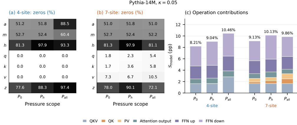
Figure 10: Pressure-scope effects at the moderate threshold \kappa = 0.05 . The six 14M recipes use the same count pooling and operation denominator as Figure 6. H-only pressure concentrates zeros at h while preserving a different pattern at m and Q/K/V from broad pressure. Rounded percentages do not establish all-zero or fully dense tensors.
