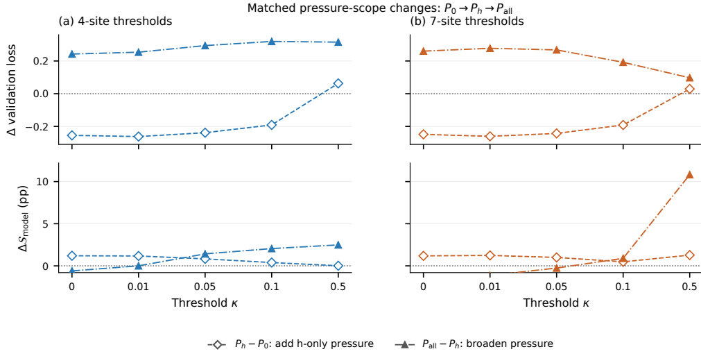
Figure 4: The marginal effect of pressure depends on its scope and the threshold. Columns hold four- or seven-site thresholding fixed. Each point subtracts the reference at the same \kappa : diamonds show P_h - P_0 , triangles show P_{all} - P_h . The top row reports validation-loss change and the bottom row model-wide sparsity change in percentage points. Lines join separately trained, matched settings, not training trajectories. Each condition has one seed, with matched initialization, data order and training budget.
