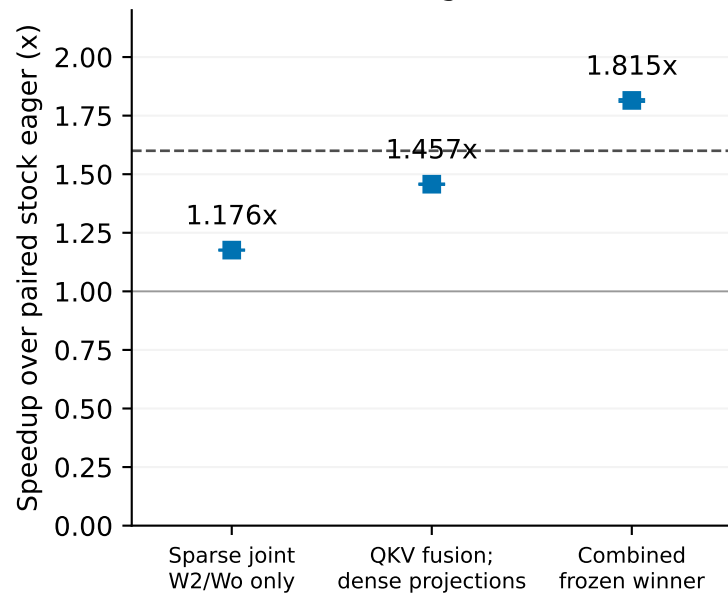
Held-out timing + ablations
