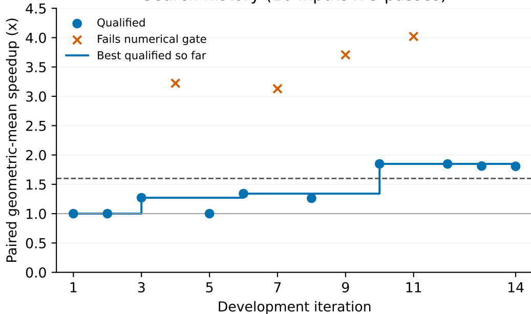
Search history (16 inputs x 5 passes)
