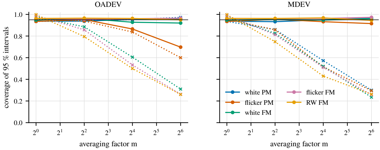
Figure 2: Share of 400 simulated records in which the 95% interval contains the true deviation. Solid: \chi^2 intervals with the exact discrete EDF and the noise type identified from each record. Dotted: the shortcut \sigma \pm 1.96 \sigma / \sqrt{n} . The horizontal line marks 0.95.
