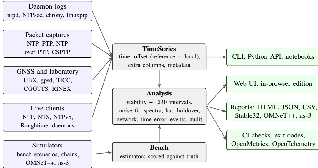
Figure 1: Structure of ntpstats . Every input is converted to one series type with one sign convention; the analysis and the bench operate only on that type, and every result is available through the command line, the Python API, the web interface and machine-readable reports.
