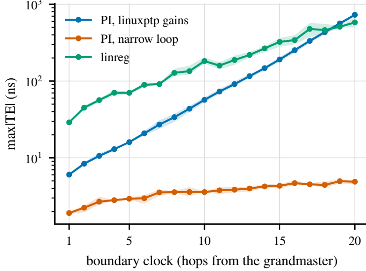
Figure 5: \max|TE| of each boundary clock along a 20-hop chain (mean of three seeds; the band spans the seeds). Default linuxptp gains show gain peaking: the error grows much faster than the number of hops.
