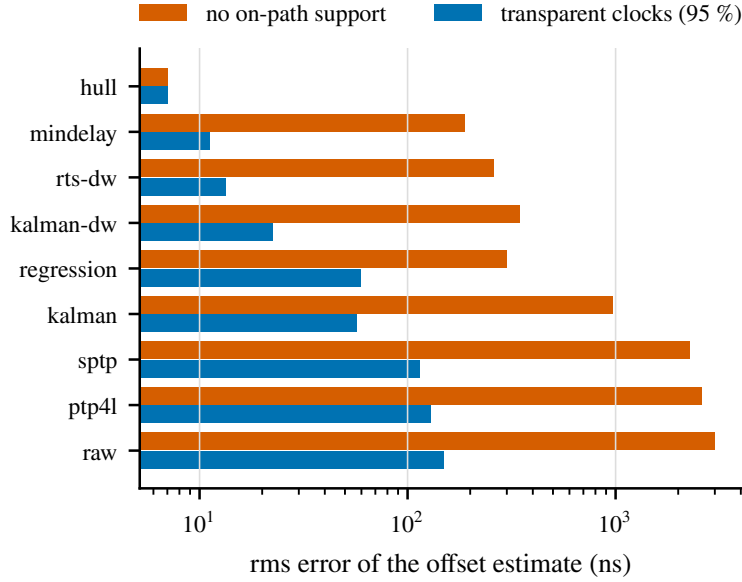
Figure 4: RMS error of the offset estimate on exchange-level PTP, without on-path support and with transparent clocks that correct 95% of the queueing (three seeds, 4 h each).
