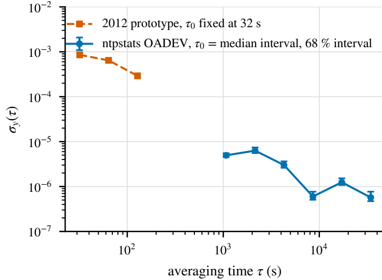
Figure 3: Stability of the 2012 sample loopstats file: the 2012 prototype, which fixed \tau_0 = 32 s, against ntpstats OADEV with the median interval, gaps left open and 68% intervals.
