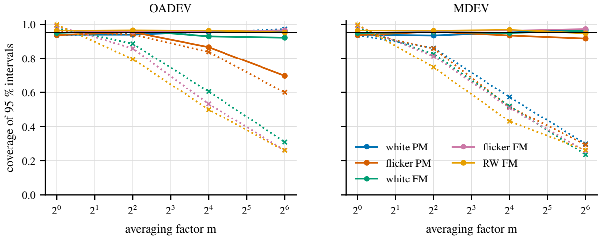
Figure 2: Share of 400 simulated records in which the 95% interval contains the true deviation. Solid: \chi^2 intervals with the exact discrete EDF and the noise type identified from each record. Dotted: the shortcut \sigma \pm 1.96 \sigma / \sqrt{n} . The horizontal line marks 0.95.
