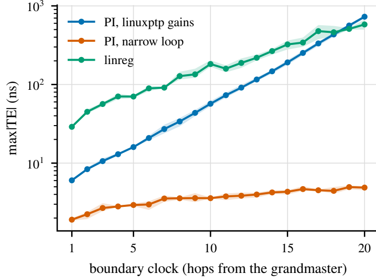
Figure 5: \max|\text{TE}| of each boundary clock along a 20-hop chain (mean of three seeds; the band spans the seeds). Default linuxptp gains show gain peaking: the error grows much faster than the number of hops.
