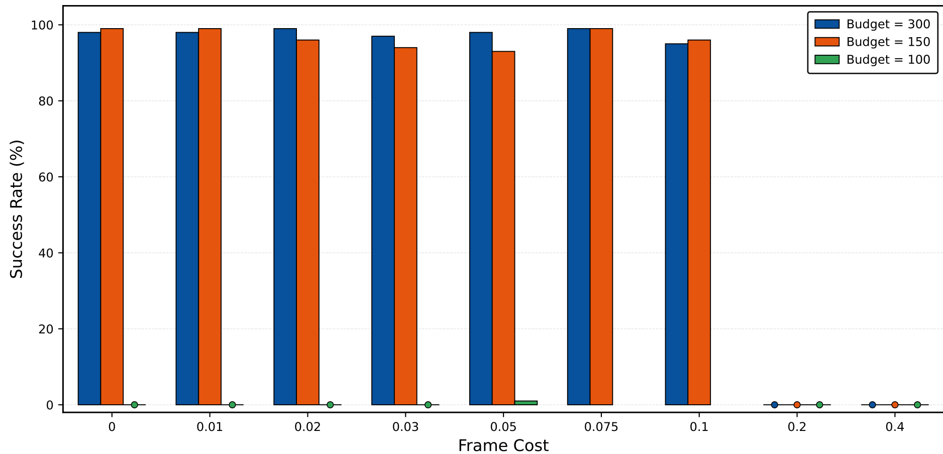
Success Rate vs. Frame Cost
