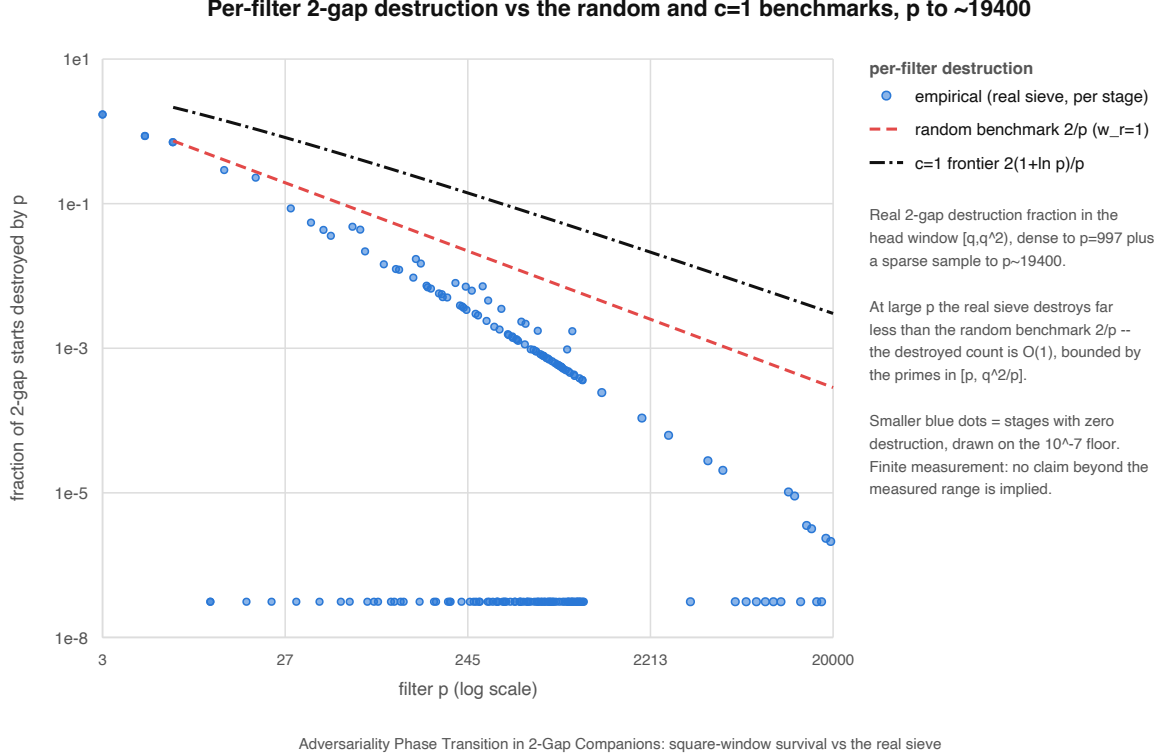
Figure 6: Real per-transition square-window 2-gap destruction compared with the random rate and the c=1 square-window boundary
