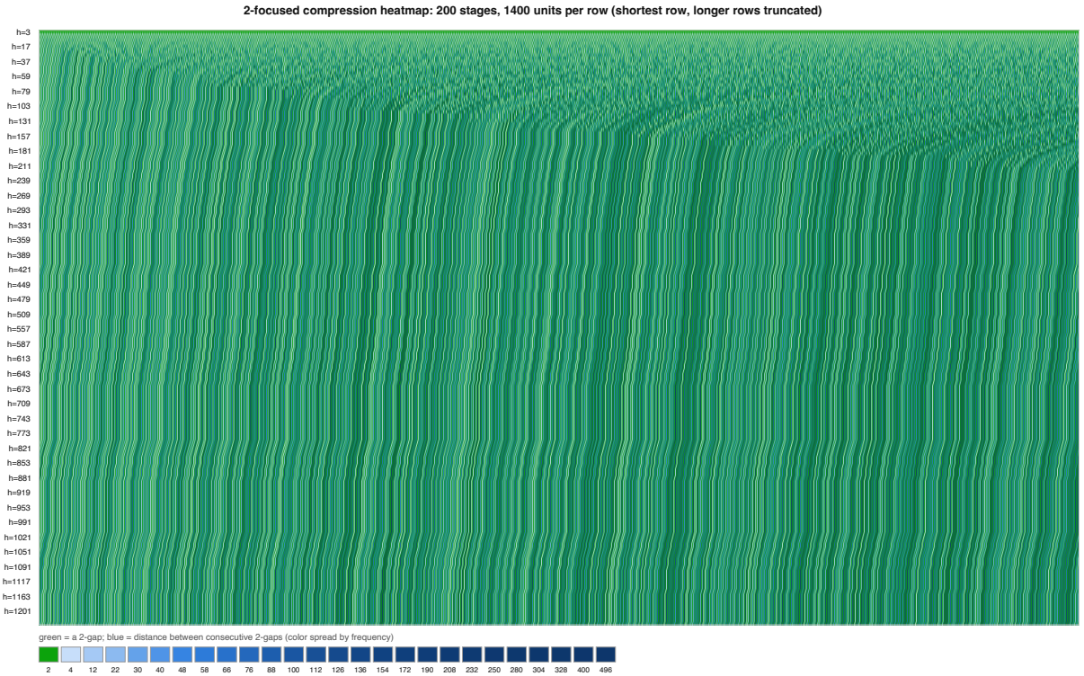
Figure 1: Independent 2-focused snapshots of 200 Sieve Sequence stages: every row restarts at its own head
