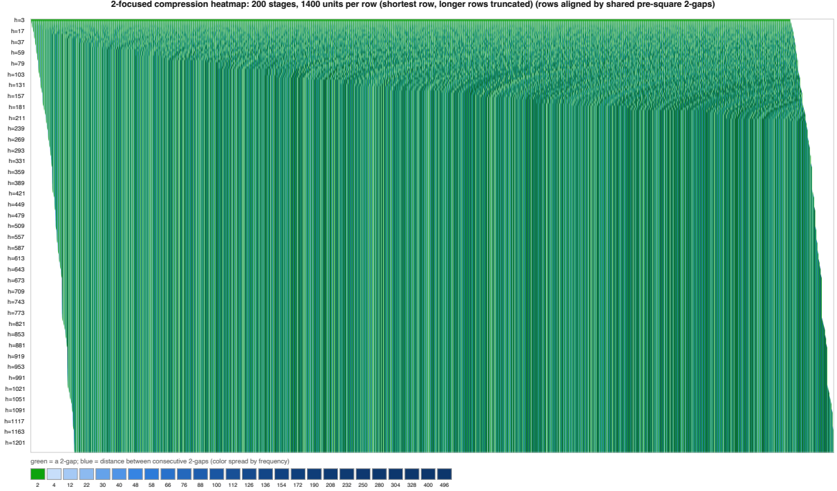
Figure 2: Shared-safe-2 aligned compression of 200 Sieve Sequence stages: unchanged pre-square 2-gaps form vertical green lines
