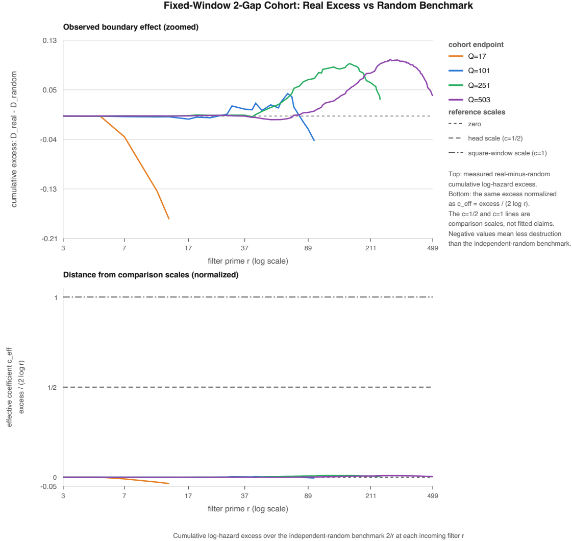
Figure 9: Cumulative hazard of fixed-window 2-gap cohorts for four finite Q values
