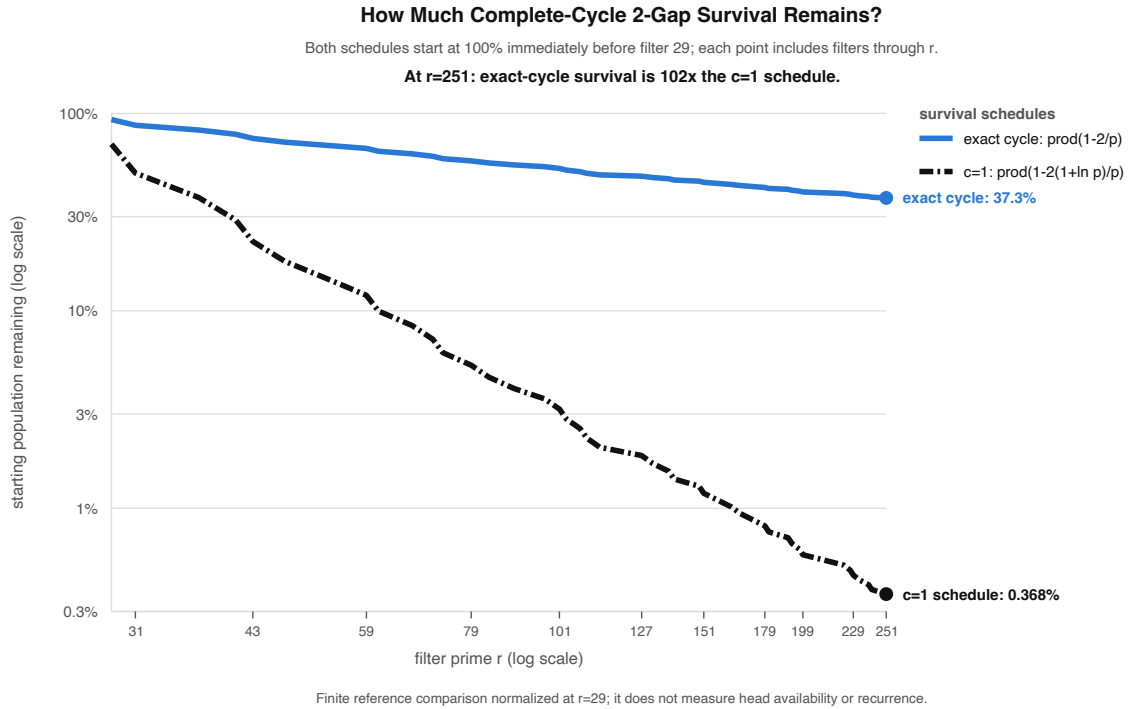
Figure 8: Normalized full-cycle 2-gap survival under the exact per-filter law compared with the c=1 schedule
