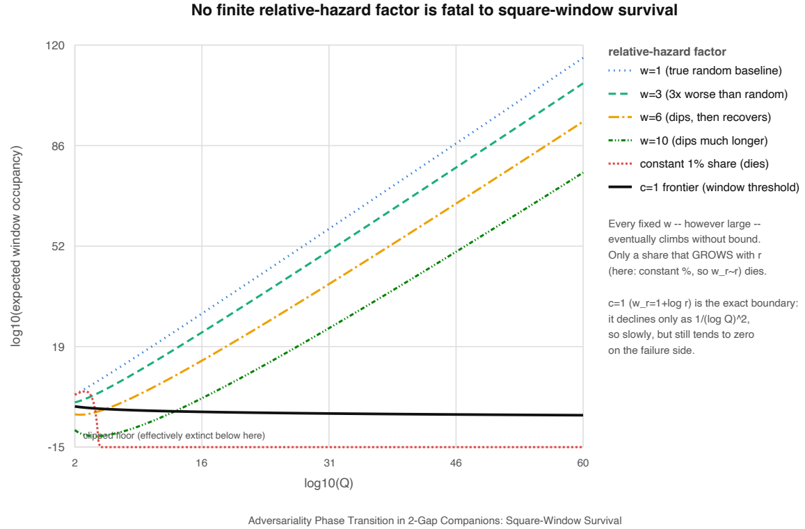
Figure 3: Square-window expected occupancy \log_{10}(\lambda(Q)) on a log scale: every fixed relative-hazard factor w=1,3,6,10 eventually climbs without bound, a constant 1% adversarial share collapses rapidly, and the exact c=1 boundary declines slowly to zero
