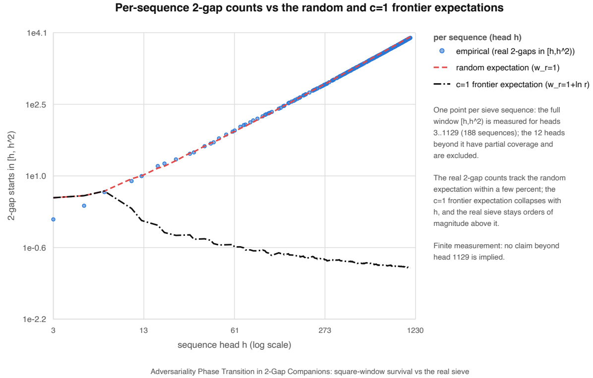
Figure 5: Real per-sequence square-window 2-gap counts compared with the random expectation and the c=1 square-window frontier
