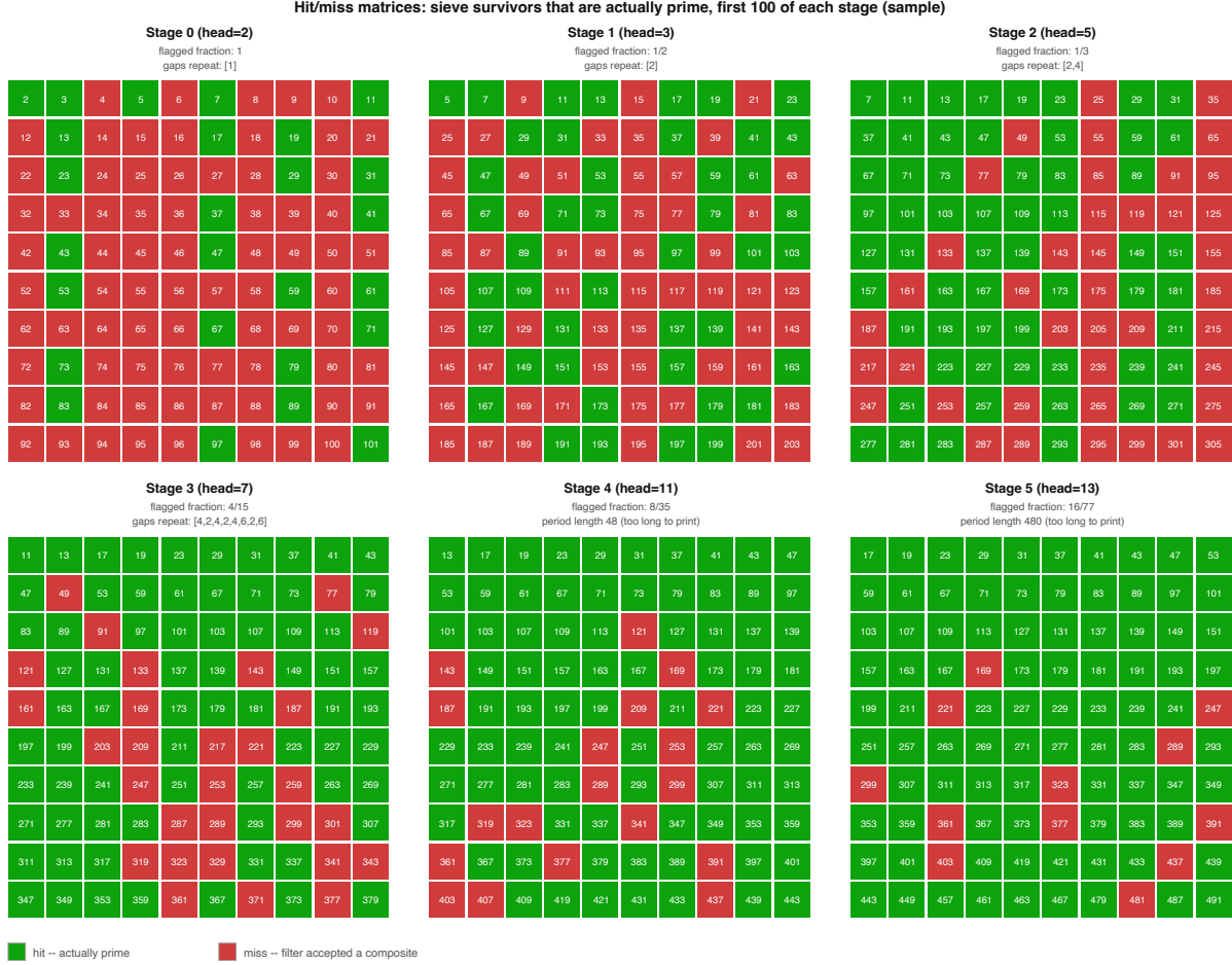
Figure 1: Six small hit/miss matrices, one per early stage: green cells are survivors that are actually prime, red cells are survivors the current filter set accepted anyway even though they are composite.
