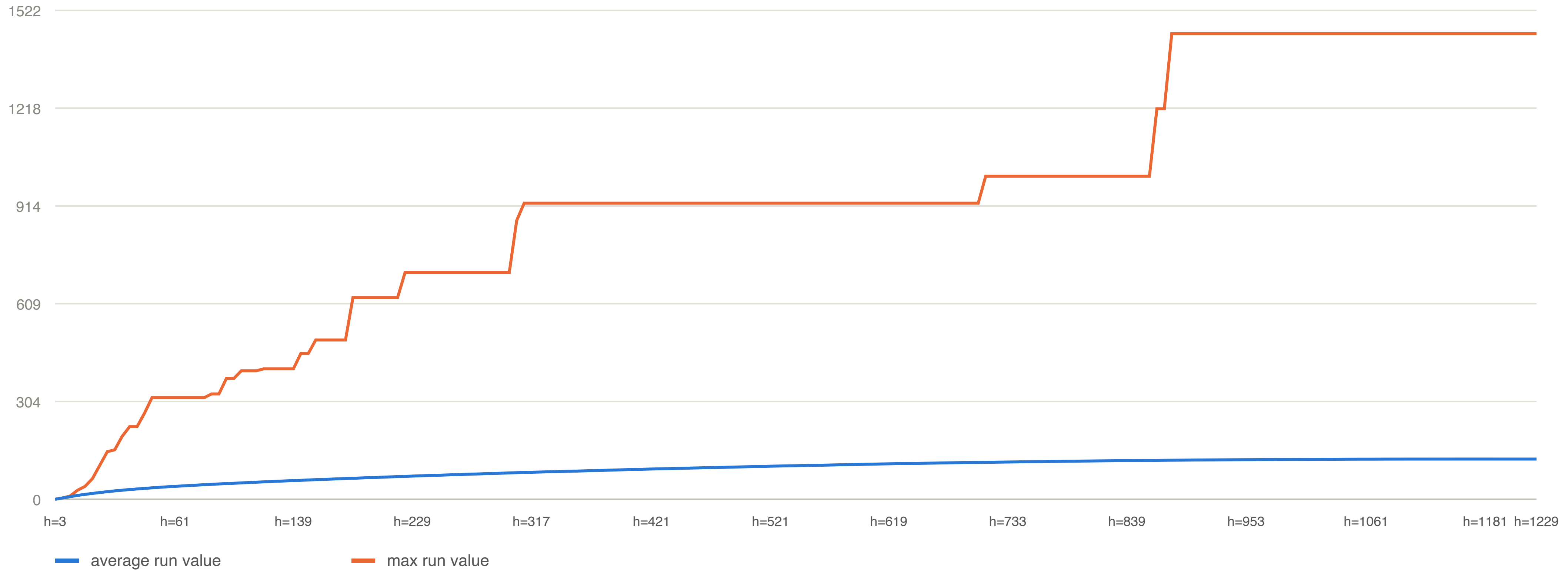
2-gap cluster size: typical (avg) and largest (max) distance between consecutive 2-gaps, per stage (200 stages)
