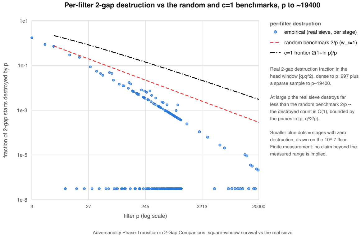
Figure 6: Real per-transition square-window 2-gap destruction compared with the random rate and the c=1 square-window boundary
