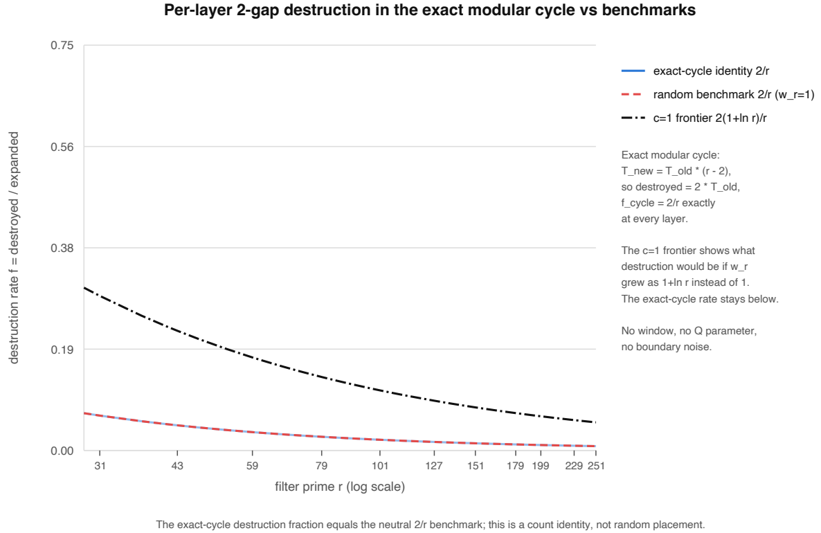
Figure 7: Exact full-cycle 2-gap destruction fraction compared with the neutral rate and the c=1 reference
