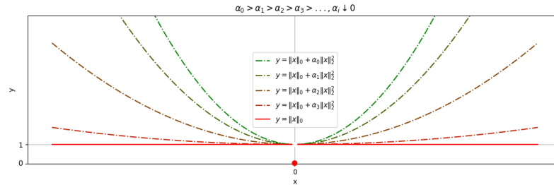
Figure 1: l_0 l_2 towards l_0 .
