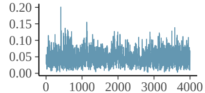
mu_lambda_recency
