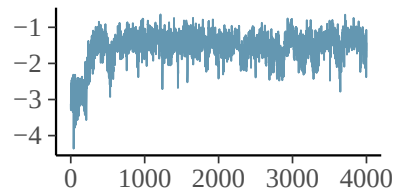
mu_pr[7]
