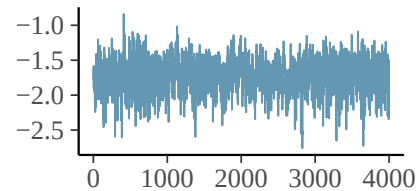
mu_pr[1]
