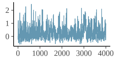
mu_pr[4]
