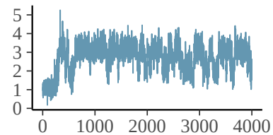
mu_pr[5]
