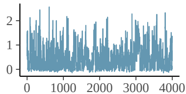
mu_pr[2]
