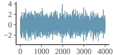
mu_pr[3]
