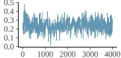
mu_pr[6]
