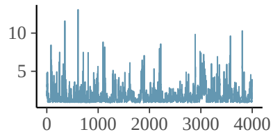
mu_Delta_plus
