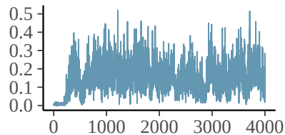
mu_sigma_rep
