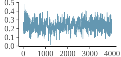
mu_l_anchor
