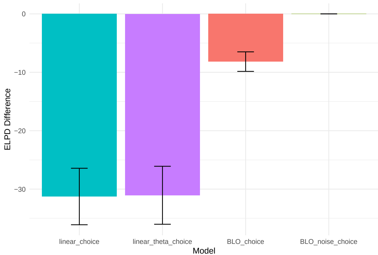
Model Comparison: ELPD Difference with Error Bars
