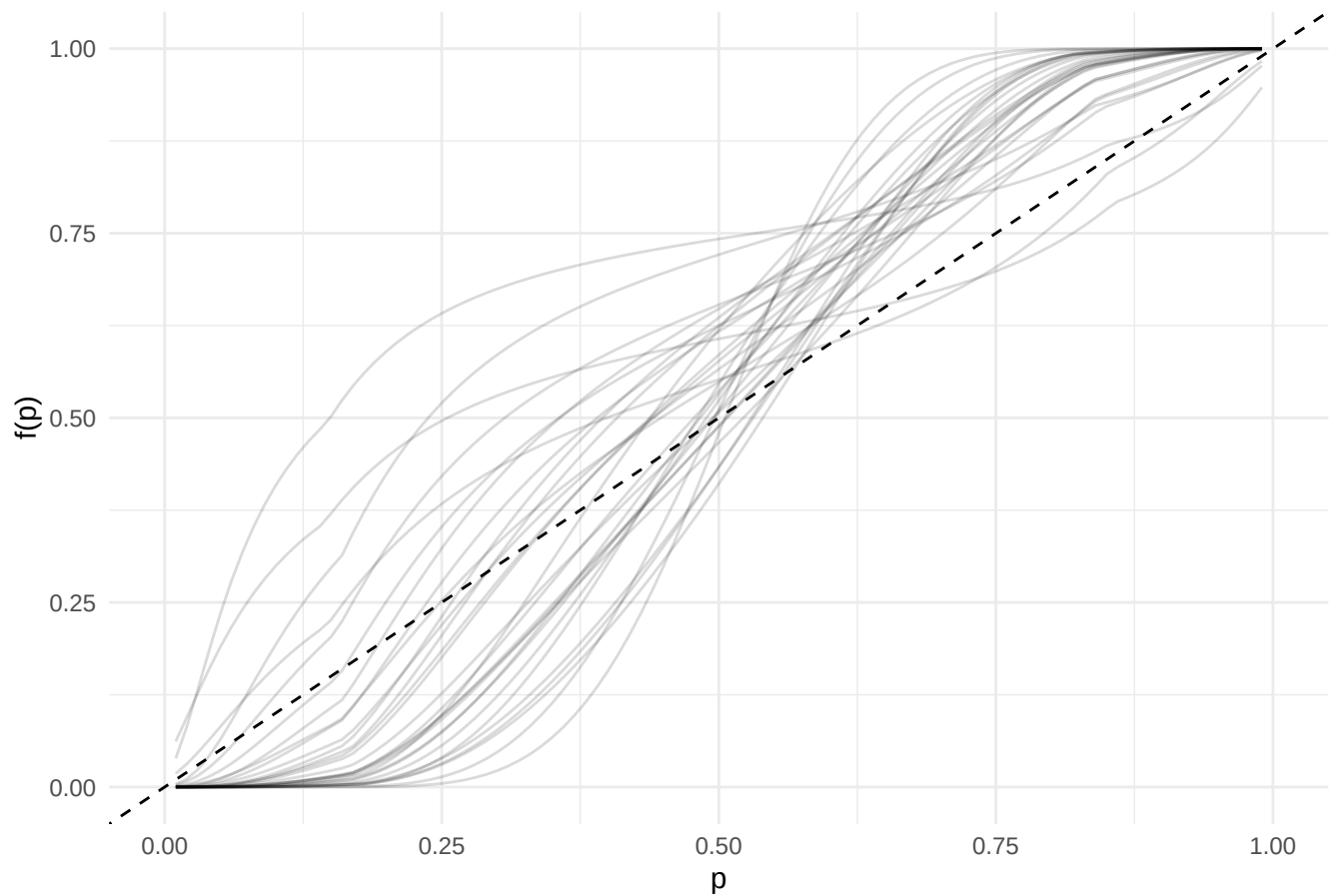
Probability transformation – individuals (BLO_noise_choice, exp17)
