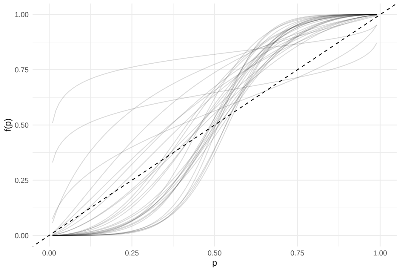
Probability transformation – individuals (linear_theta_choice, exp17)
