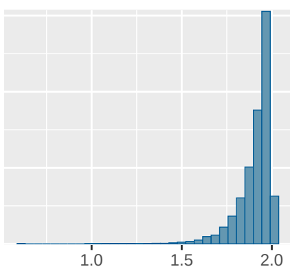
mu_alpha
