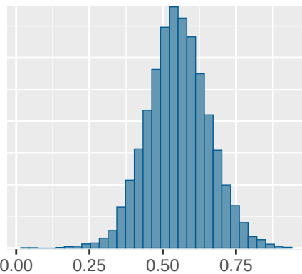
mu_beta
