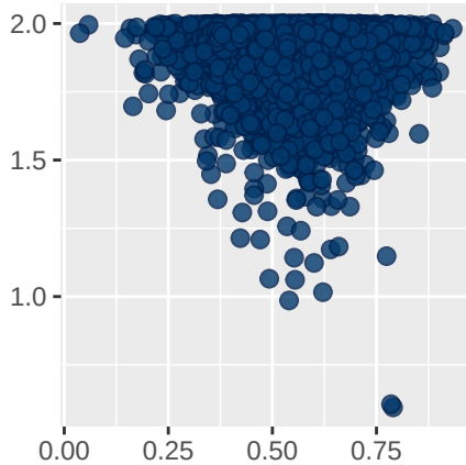
mu_beta
