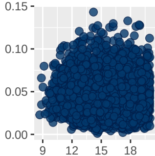
\mu_{\theta}
