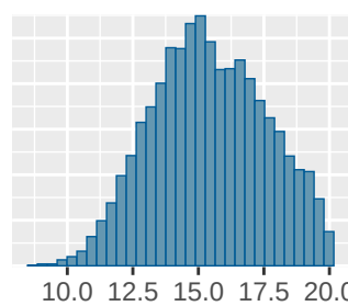
\mu_{\theta}
