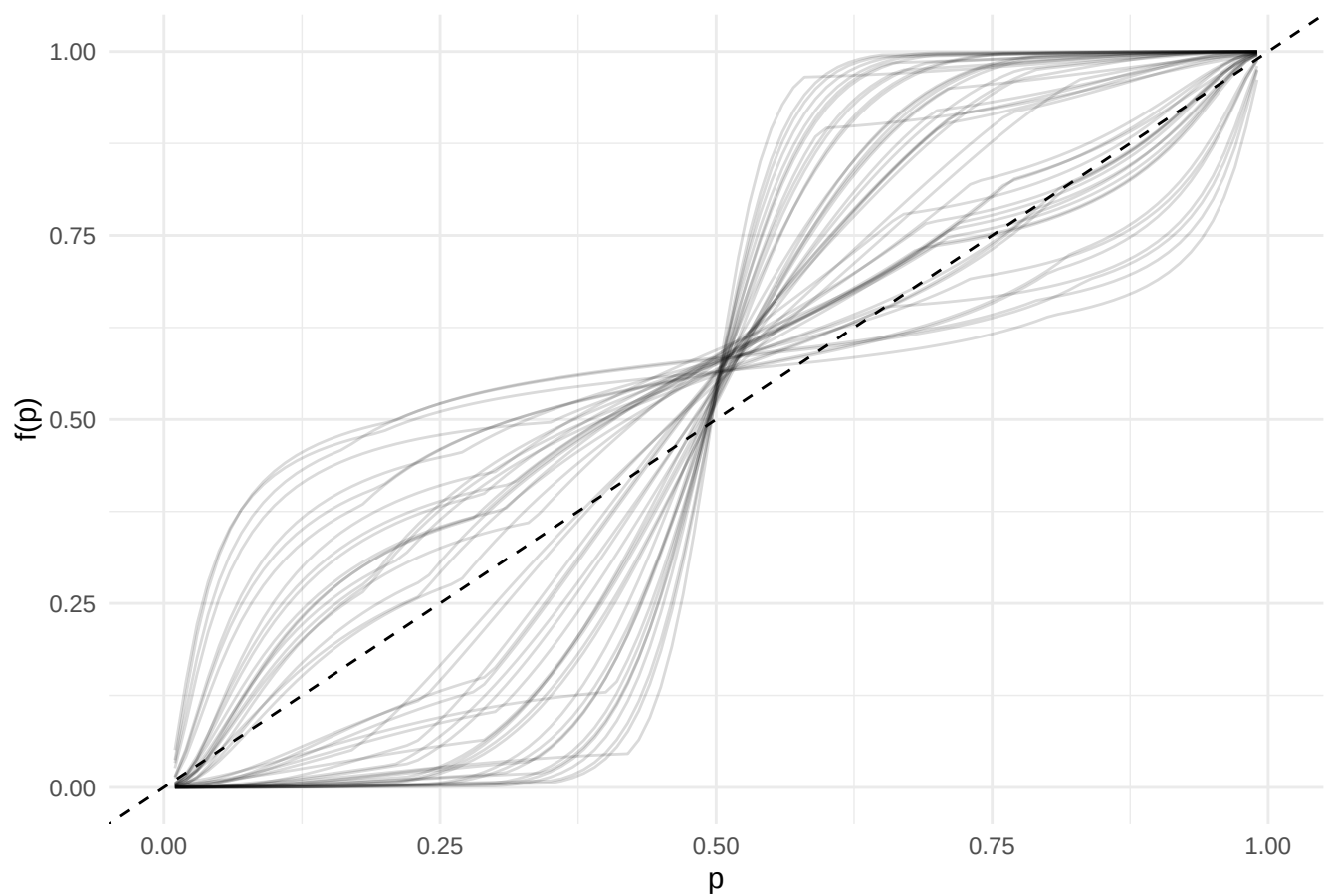
Probability transformation – individuals (BLO_noise_choice, exp8)
