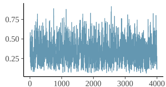
mu_beta
