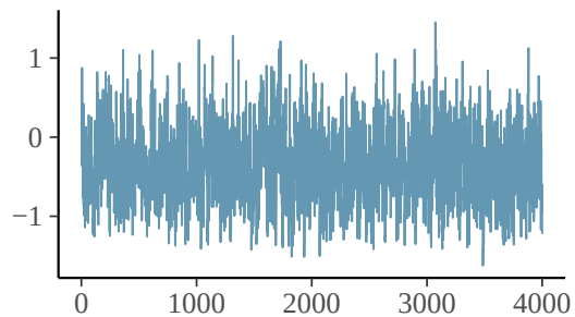
mu_pr[2]
