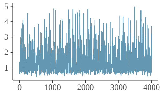
mu_theta
