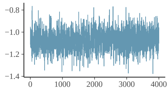
mu_pr[1]
