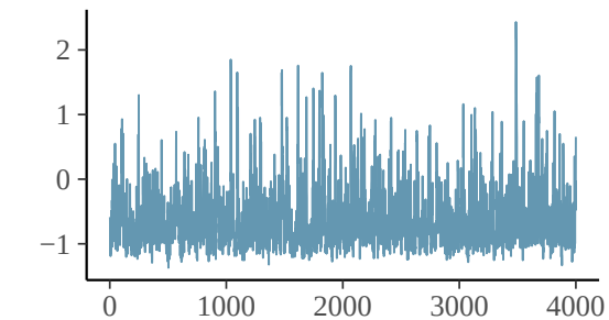
mu_pr[4]
