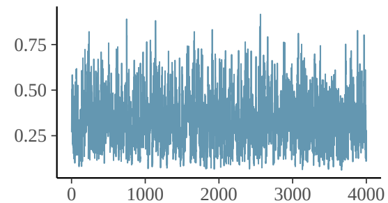
mu_pr[3]
