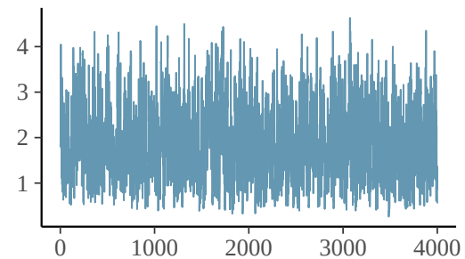
mu_alpha
