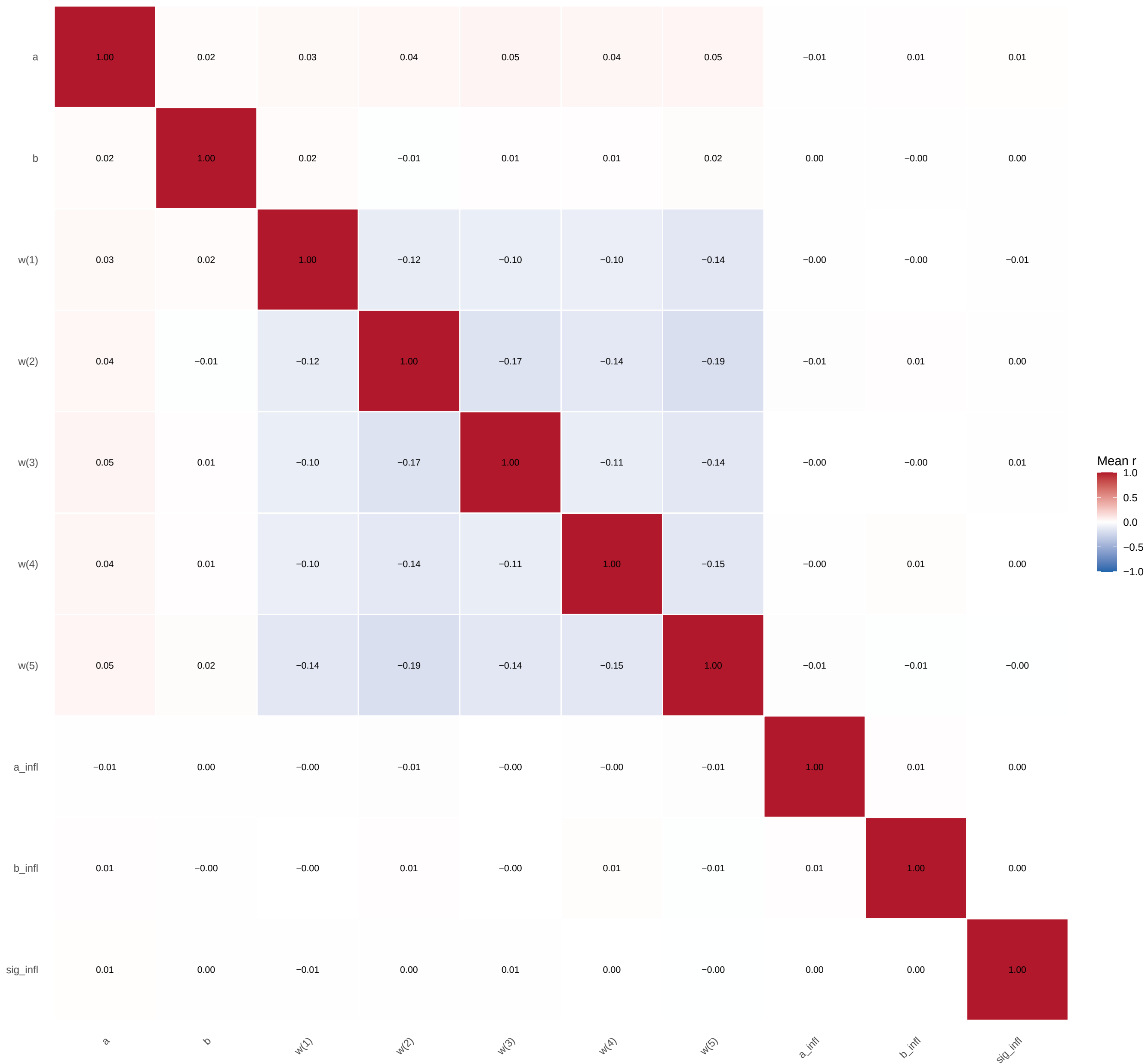
Mean parameter correlations (across 705 fits)
