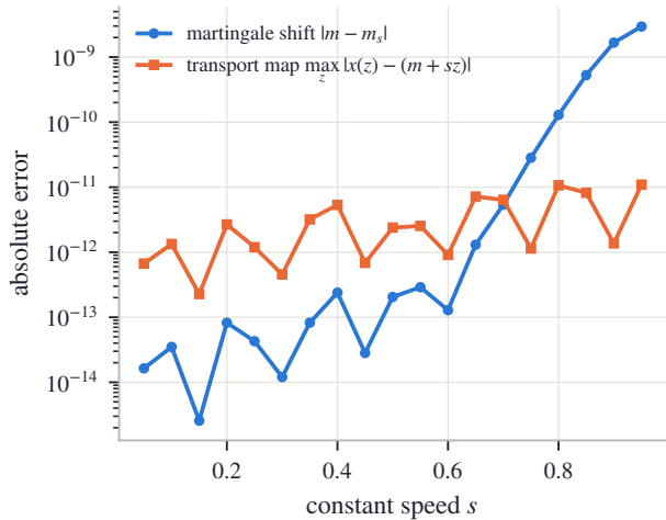
(a) error against m_s = -\log \frac{\pi s}{\sin \pi s}
