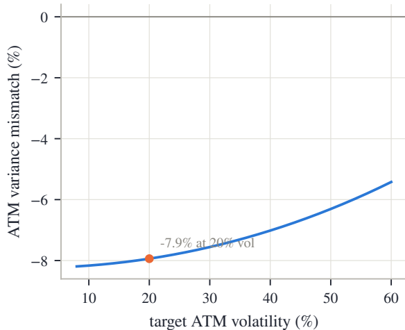
(b) the variance-matched cold start
