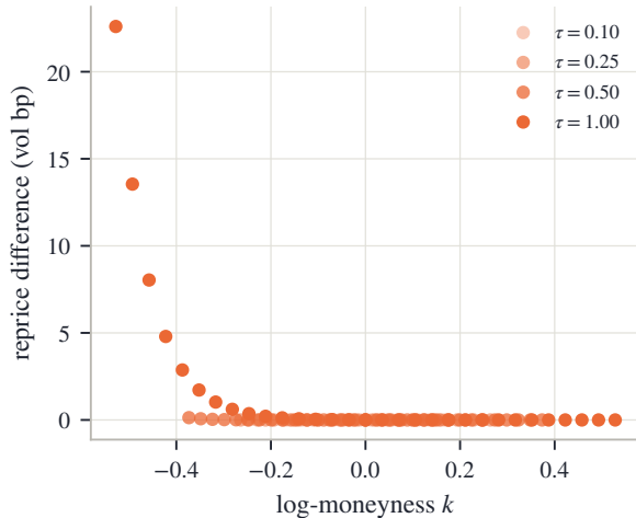
(b) what the quote set notices
