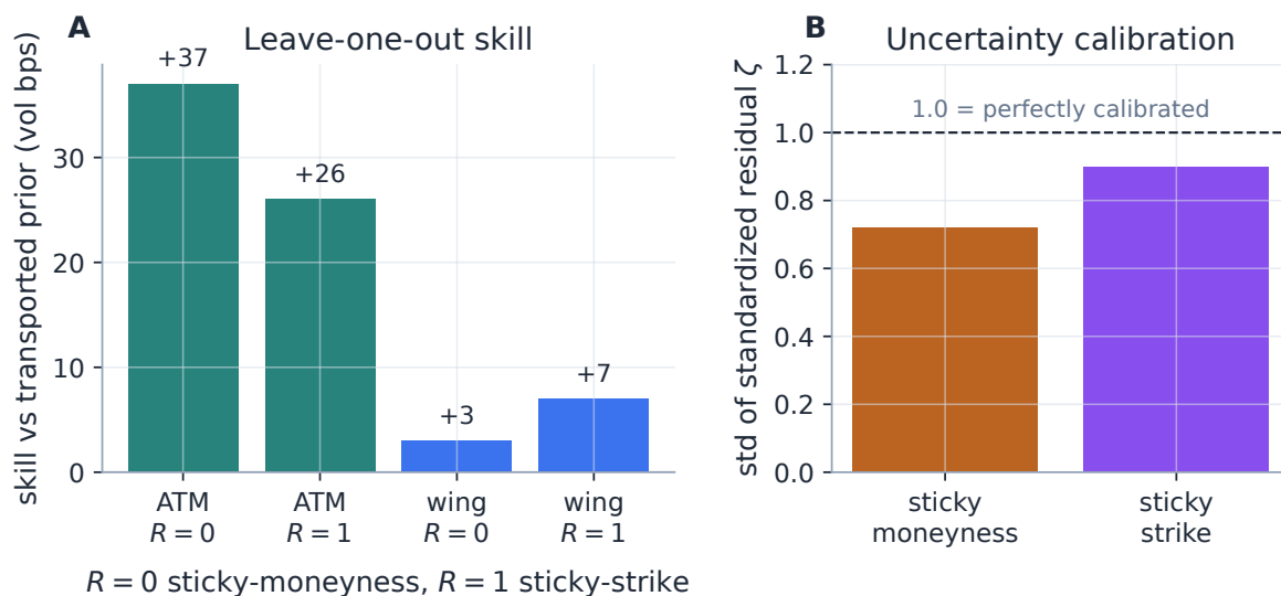
Figure 5: The leave-one-out verdict. Left: skill over the transported prior for the headline use case, bracketed by the two transport regimes — the graph adds +25.6 to +37.1 ATM vol bps. Right: the standardized-residual std is below one in both regimes: the posterior bands are slightly conservative, never overconfident.
