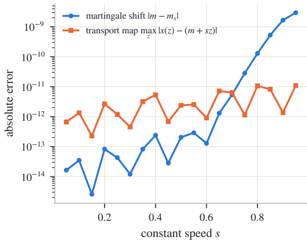
(a) audit against m_s = -\log \frac{\pi s}{\sin \pi s}
