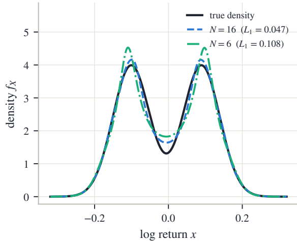
(b) where the missing order went
