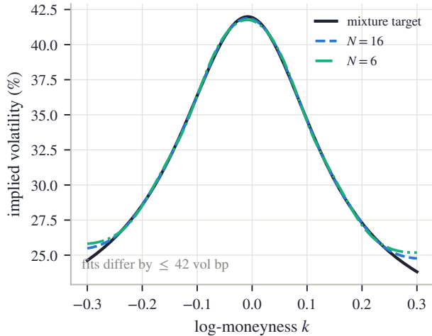
(a) two orders, almost one smile
