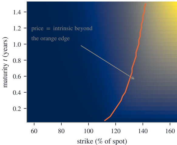
(a) puts, r = 4\% , no dividends
