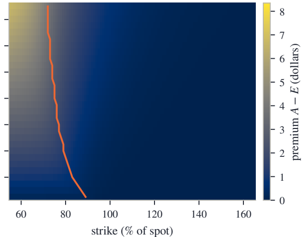
(b) calls, q_d = 6\% against r = 2\%
