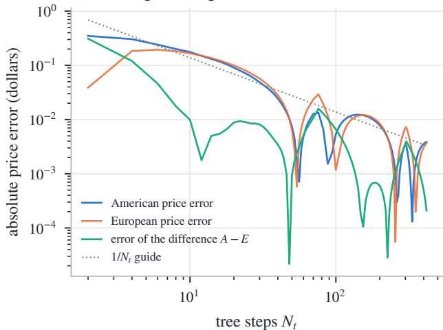
(b) both legs converge like 1/N_t ; their difference is cleaner
