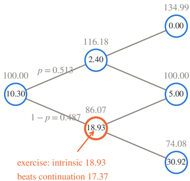
(a) the two-step American put (spot above, value below)
