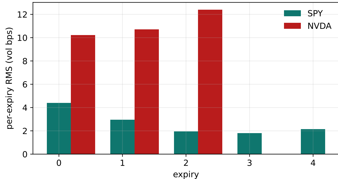
Production local-vol fit, Bloomberg fixture
