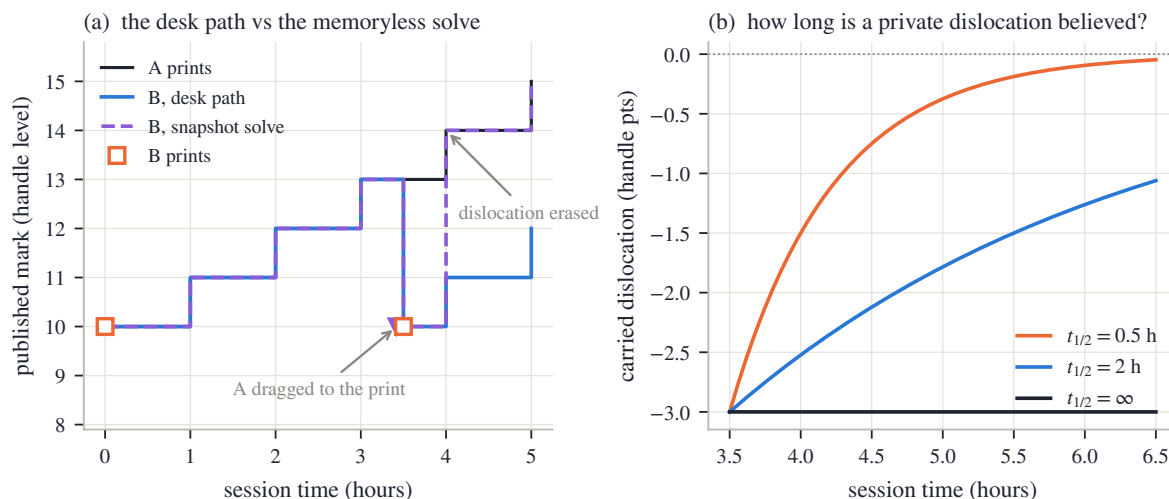
Figure 11.6: The asynchronous pair. (a) A prints hourly (ink); B prints twice (orange squares). The desk path (blue) rides the relation between prints, learns the -3 -point dislocation at the 3.5-hour print, and keeps it: 14 - 3 = 11 at hour 4. The per-instant solve (dashed violet) drags A to the print at hour 3.5 (no direction) and erases the dislocation at hour 4 (no memory). (b) The carried dislocation under three half-lives: what t_{1/2} asserts is how long a private dislocation stays believed.
