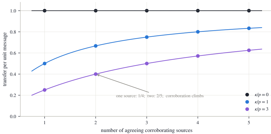
Figure 11.5: The corroboration law eq. (11.6): transfer per unit message against the number of agreeing sources, for anchor settings \kappa/p = 0 (full force), 1 (half through at one source) and 3 (a quarter through at one source). Curves are the law; dots are the chapter’s solver, agreeing to 2.5 \times 10^{-9} . Corroborating voices climb through the anchor; the anchor never touches the relation itself.
