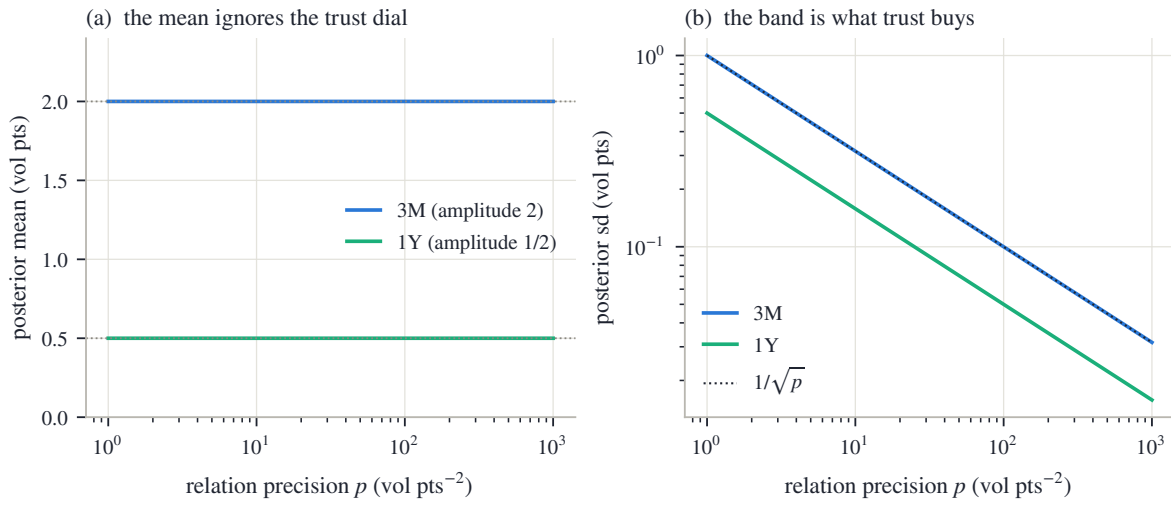
Figure 11.2: The contract on the clean ladder (3M/6M/1Y, 6M lit at +1 volatility point, calendar amplitudes eq. (11.2)). (a) Posterior means at the two dark nodes against the relation precision: flat at the configured +2.00 and +0.50 across three decades (maximum deviation 3.3 \times 10^{-9} ). (b) Posterior standard deviations: falling as 1/\sqrt{p} (dotted), with the 1Y band exactly half the 3M band — the same relation noise read in 1Y units. Amplitude prices the mean; trust prices the band.
