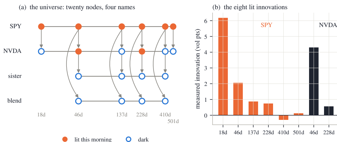
Figure 11.1: The staged universe. (a) Twenty nodes in four rows: the real SPY and NVDA boards (six expiries each) and two synthetic names built from them. Filled orange nodes are lit this morning (8 of 20); open nodes are dark. Grey segments are calendar edges within a name; arrows are cross-name edges, pointing from the informing name to the informed one. (b) The eight lit innovations: each lit node’s calibrated handle minus its transported baseline, in volatility points. The morning is a broad repricing, largest at the short end.
