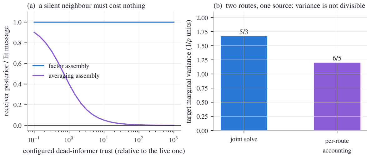
Figure 11.4: Two accounting tests. (a) The silent neighbour: the factor assembly transfers the whole lit message no matter how much trust the dead informer carries (blue, flat at 1.0000); the averaging assembly (violet) leaves the posterior improper, and a vanishing ridge then retains only 0.40 at equal trust, decaying toward zero. (b) One source, two routes: the joint solve prices the target's variance at 5/(3p) ; treating the two routes as independent messages yields 6/(5p) — a 39% precision overstatement, because both routes share the source's own doubt.
