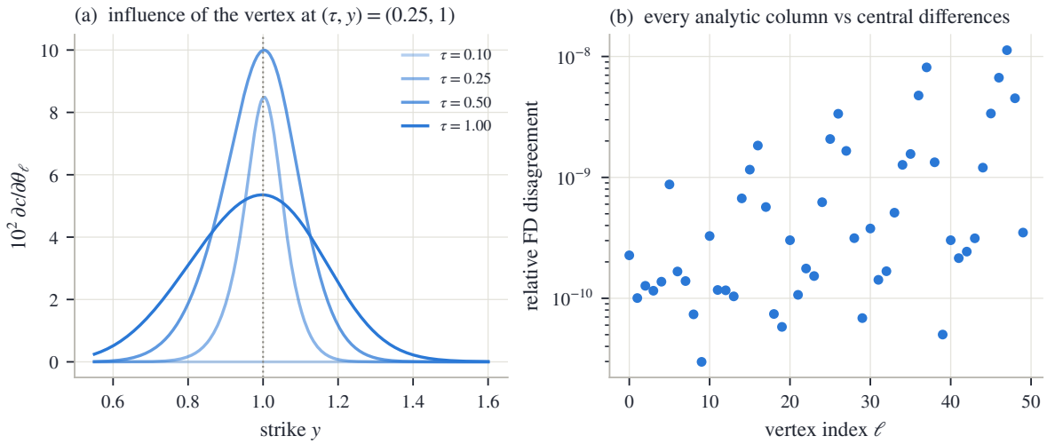
Figure 4.7: The tangent system, seen and checked. (a) Sensitivity of the priced call curve to the single vertex at (\tau, y) = (0.25, 1) , across the four quoted expiries. (b) Every analytic column of the Jacobian against a central finite difference of the full march, over all 50 vertices: worst relative disagreement 1.1 \times 10^{-8} .
