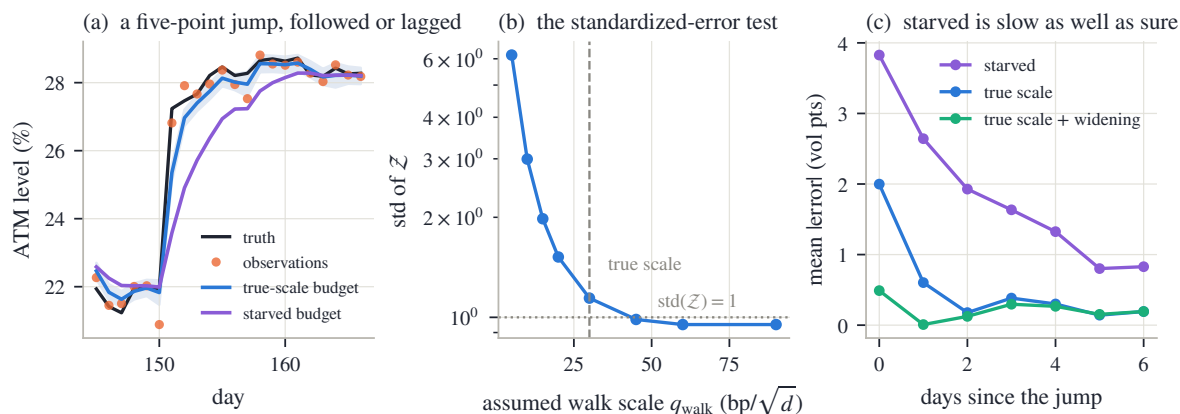
Figure 10.7: The standardized-error test on a seeded synthetic history (500 days; the true level diffuses at 30 \text{ bp}/\sqrt{\text{day}} and jumps +5 points twice; the filter is told the true observation noise, wide on every seventh day). (a) A window around a jump: the filter run at the true walk scale (blue, with its \pm 1 -sd band) follows in two days; the starved budget (violet) crawls. (b) The test curve: std of Z against the assumed walk scale — starved budgets sit far above the dotted target of 1 (3.0 at 10 bp), the true scale reads 1.14. (c) Mean error against days since the jump: starved 3.8 points on the day and still 1.6 three days later; the true scale 2.0 then pennies; the surprise widening cuts the jump-day error to 0.49.
