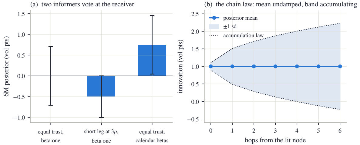
Figure 11.3: Messages meeting. (a) The 6M receiver hears its lit neighbours at \pm 1 volatility point, three ways: equal trust at amplitude one (exact cancellation, under a band tighter than either informer alone would leave — precisions added even as the means cancelled); the short leg at 3p (the louder voice wins, -0.50 ); equal trust under calendar amplitudes (the same signals map to -0.5 and +2 in receiver units before averaging: +0.75 ). Whiskers are \pm 1 posterior sd. (b) A six-hop chain, far end lit at +1 : the mean crosses every hop undamped while the band accumulates exactly the chain law eq. (11.4) (dotted).
