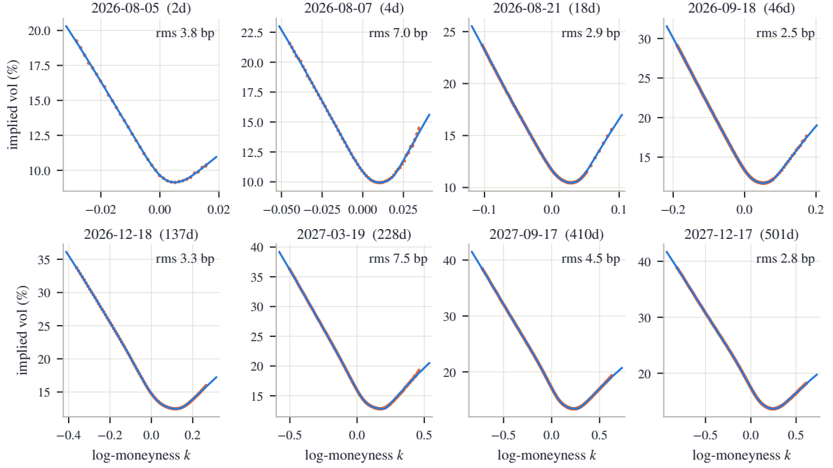
Figure 2.10: Eight SPY expiries fitted with one recipe. Each panel shows raw bid–ask quotes, mids, the fitted LQD slice, and rms error. The short end is steeper and more localized; the long end broadens smoothly. Beyond the last quote, each curve is determined by the fitted exponential-tail convention.
