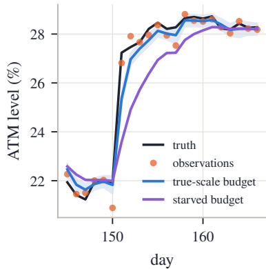
(a) a five-point jump, followed or lagged
