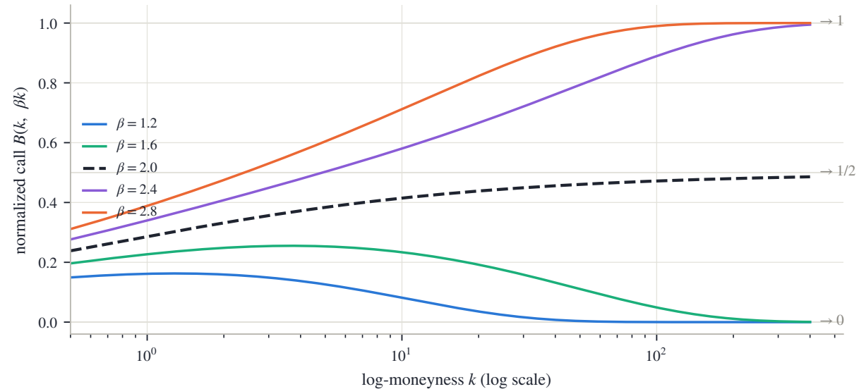
the far-out-of-the-money call along rays of slope \beta
