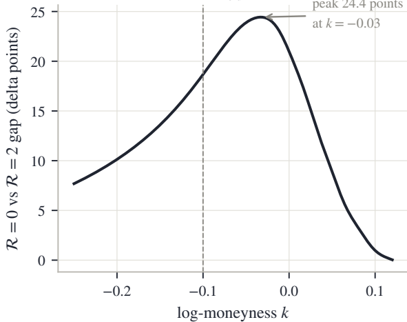
(b) the gap 2\varphi(d_+) \sqrt{t} |\sigma'_{\text{old}}(k)|
