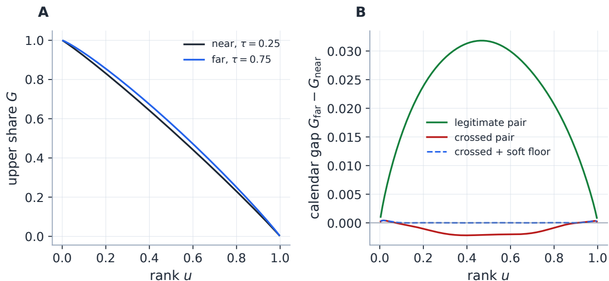
Figure 9: Convex order on the ledger, three ways. Panel A: upper shares of a legitimate near/far pair (the running example and a proportionally scaled quarter-year slice) — both start at the common mean and the far curve dominates. Panel B: the calendar gap G_{\text{far}} - G_{\text{near}} . Green: the legitimate pair stays non-negative (minimum 0.00087). Red: a crafted far slice whose body variance sits below the near slice dips to -0.00218 near the u \approx 0.39 rank — calendar arbitrage a strike-space inspection of two decent-looking smiles would not shout about. Dashed blue: the same crossed quotes refitted with the production soft floor; the violation collapses to -3.45 \times 10^{-6} — pressed against zero from below, visibly soft, visibly working.
