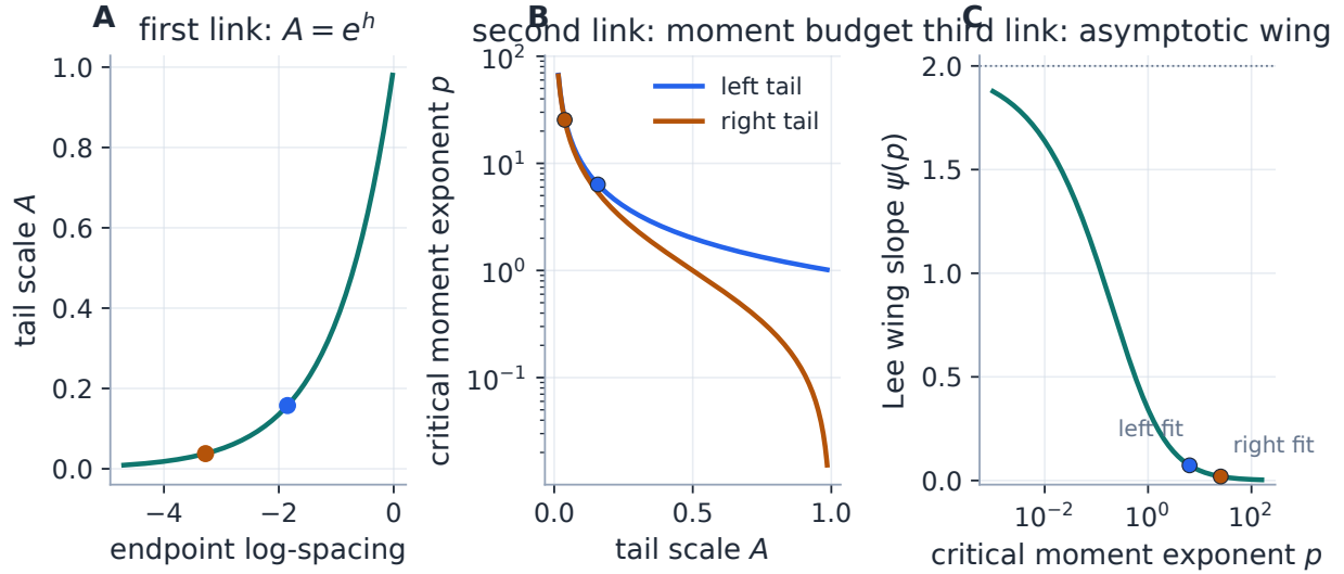
Figure 11: The fitted tails walked through the three links of section 4: endpoint value of g to tail scale ( A_L = 0.157473 , A_R = 0.037786 ), tail scale to last finite moment (13), and moment to Lee wing slope (16) ( \beta_L = 0.073087 , \beta_R = 0.019259 ). Nothing imposed these wings; they are what the quoted body implied through the basis.
