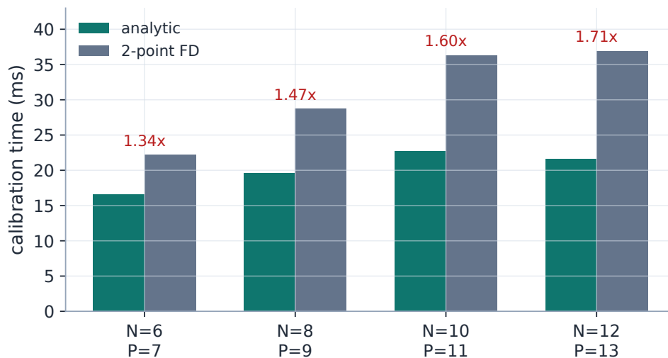
Figure 8: The same measurement drawn: per-fit wall time with the analytic one-pass Jacobian vs the (P+1) -rebuild finite difference, with the ratio above each pair. The win grows with the parameter count, as it must — the analytic pass costs one quadrature regardless of P .
