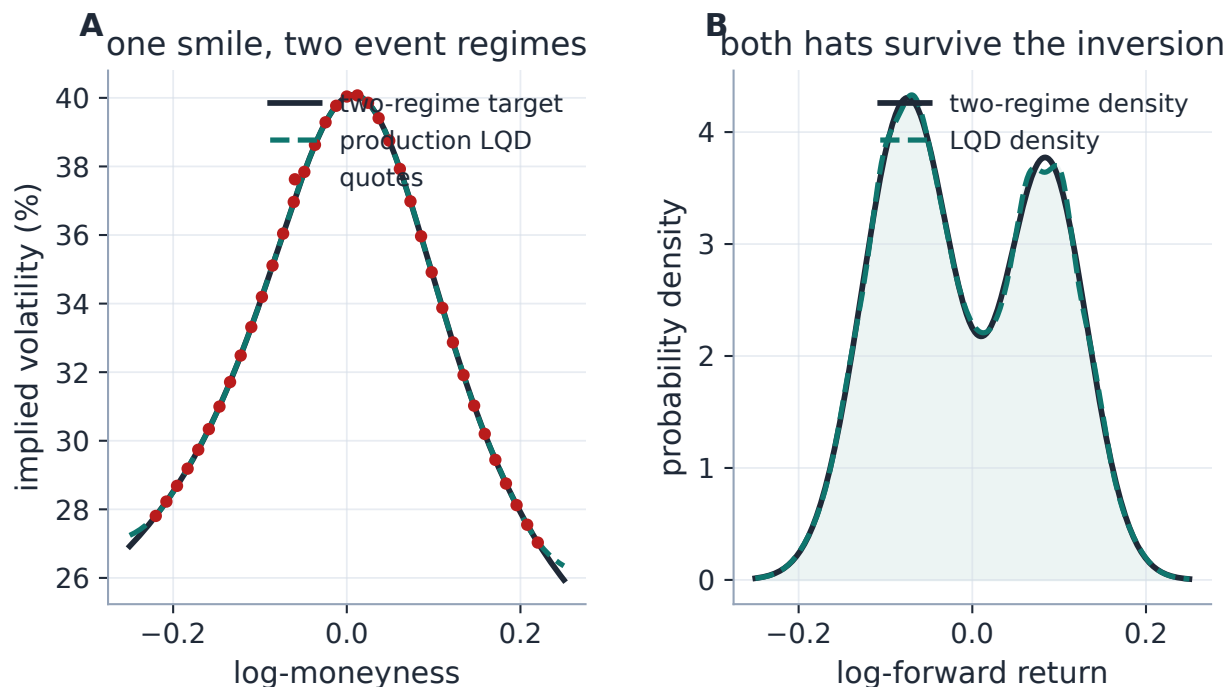
Figure 12: The event case. Panel A: the two-regime target smile and the 16-mode production fit — note the W-shaped body a low-order model cannot make. Panel B: the true mixture density and the LQD density: both hats, the asymmetry, and the trough survive the round trip through option prices, with positivity never at risk.
