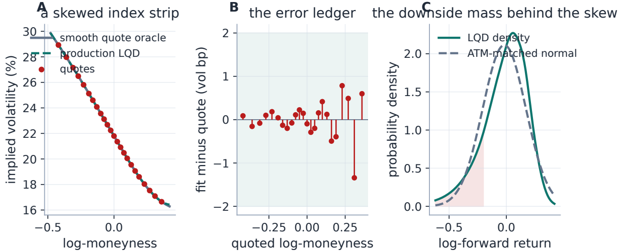
Figure 10: The SPX-like case. Panel A: quote oracle, quotes, and the production fit. Panel B: the error ledger at the quotes — every residual inside \pm 2 vol bp (shaded), maximum 1.341 vol bp against quotes carrying a deliberate \sim 2 bp ripple. Panel C: the fitted density against an ATM-matched normal: the entire content of the skew is the transfer of mass into the left tail (shaded), bought by a thinner right shoulder. Beyond the quoted window the curve is the model’s own Lee-consistent extrapolation, not an oracle continuation.
