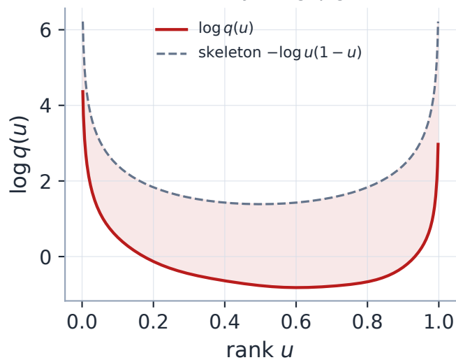
D LQD chart: only the gap g is free
