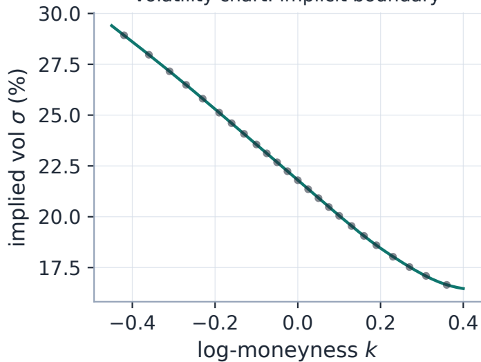
B volatility chart: implicit boundary
