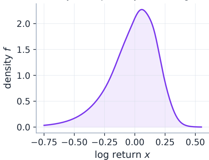
C density chart: positivity + two integrals
