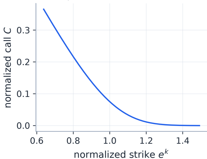
A price chart: a convex cone
