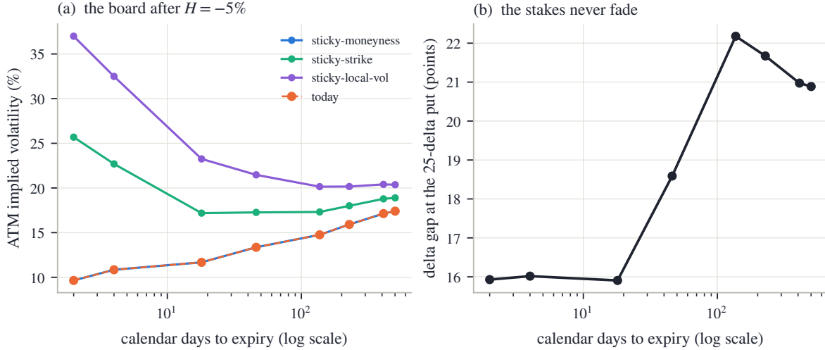
Figure 9.7: The frozen SPY board under a -5\% scenario. (a) ATM implied volatility by expiry (log time axis): today (orange, dashed) and the three transported boards. The two-day node moves from 9.6% to 9.6/25.7/37.0% under \mathcal{R} = 0/1/2 — its skew is s_0 = -2.10 . (b) The \mathcal{R} = 0 vs \mathcal{R} = 2 delta gap (9.6) at each expiry’s 25-delta put: from 15.9 delta points at two days to 22.2 at the December 2026 node and 20.9 at the far end.
