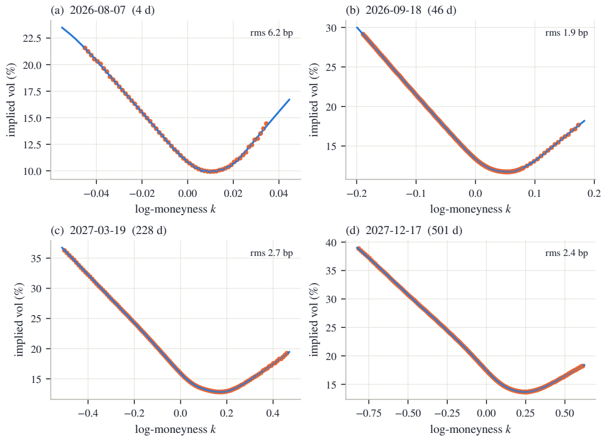
Figure 4.9: Four SPY expiries priced by the single calibrated sheet, against the frozen quotes (dots: mids; whiskers: bid–ask). Panel titles give the expiry and its distance; annotations the per-expiry rms on the fitting operator.
