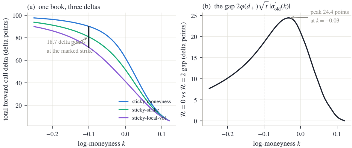
Figure 9.4: One book, three deltas (frozen hero node, eq. (9.5)). (a) Total forward call delta across strikes under the three regimes; at the marked k = -0.10 strike — a 19-delta put — the \mathcal{R} = 0 and \mathcal{R} = 2 answers are 18.7 delta points apart. (b) The gap (9.6) across strikes: the vega profile weighted by the smile's local slope, peaking at 24.4 delta points at k = -0.03 , just below the money.
