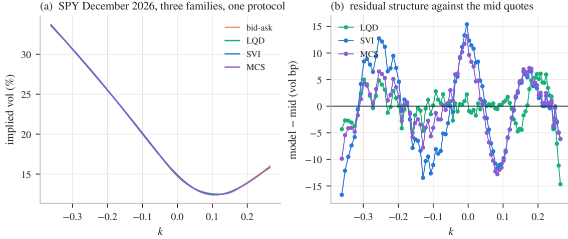
Figure 3.8: Three families, one protocol, on SPY December 2026. (a) The fitted curves overlies at chart scale inside the bid–ask band. (b) The residuals against the mid quotes separate them: LQD (3.4 bp rms, 17 parameters), MCS (5.6 bp, 14), SVI (7.5 bp, 5). More coordinates buy a whiter residual.
