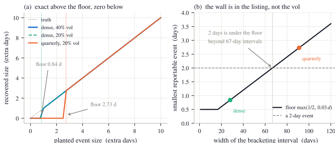
Figure 8.6: The planted-event study. (a) Recovered vs planted size on a dense board (event inside a 28-day interval) at 40% and 20% volatility, and on a quarterly board (91-day interval): exact from the floor upward (0.84 and 2.73 days), exactly zero below, identical at both volatilities. (b) The floor \max(\frac{1}{2}, 0.03 d) against the interval width d ; a two-day event clears it up to 67-day intervals.
