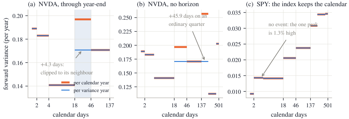
Figure 8.7: Reading the frozen boards’ clocks (forward variance per calendar year, orange, vs per installed variance year, blue). (a) NVDA with candidates through year-end: one peak, the earnings interval (shaded), clipped onto its higher neighbour by 4.3 extra days; nothing else moves; the in-horizon spread tightens from 560 to 482 variance bp. (b) NVDA with candidates everywhere: a second peak, the December-to-March quarter, is clipped by 45.9 days; 50.2 days in all, the ladder’s spread 1444 to 904 variance bp — not flat. (c) SPY: no peak clears the floor; nothing installed; the rising ladder is left standing.
