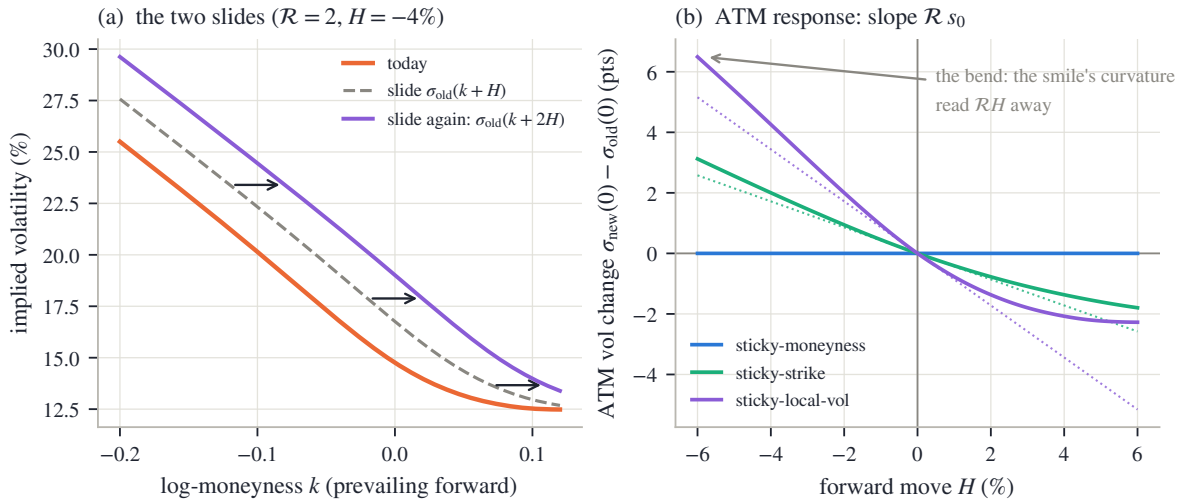
Figure 9.3: The dial (frozen hero smile). (a) The transport (9.2) for \mathcal{R} = 2 , H = -4\% , as two slides: the dashed curve is the sticky-strike slide \sigma_{\text{old}}(k + H) ; the arrows slide it once more by the same length to \sigma_{\text{old}}(k + 2H) . (b) The exact ATM response of the transport against the move for the three regimes (solid), with the linear law \mathcal{R}s_0H dotted: the slopes are \mathcal{R}s_0 , and each curve bends by the smile's curvature read \mathcal{R}H away — at H = -6\% , 54 vol bp under sticky-strike and 133 under \mathcal{R} = 2 .
