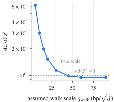
(b) the audit curve
