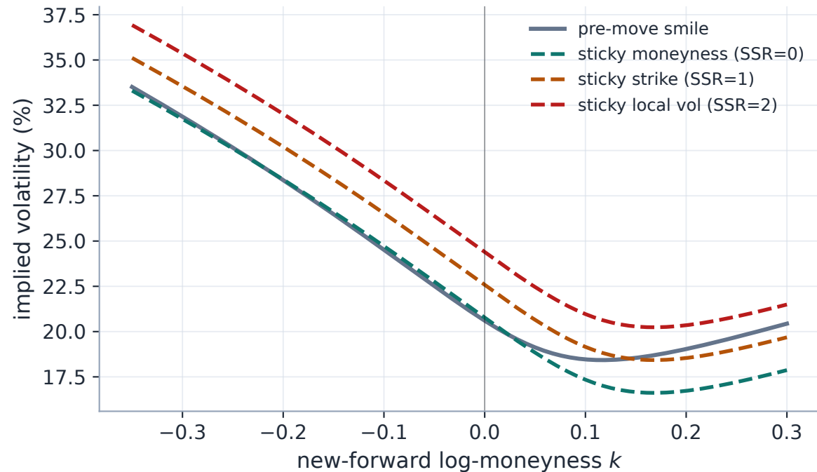
Smile after a -5\% spot move
