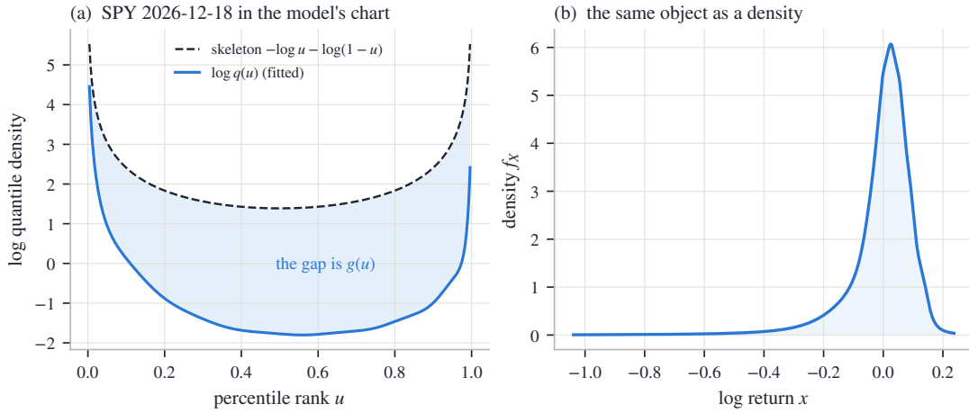
Figure 3: A fitted SPY December 2026 slice in the model's coordinates. Left: the universal boundary skeleton and the fitted \log g ; their difference is g . Right: the density produced by the same transport. The quoted strikes occupy the central ranks; the continuation to the endpoints is extrapolation.
