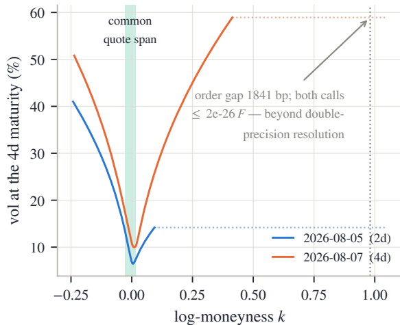
(b) the crossing lives in the empty wing
