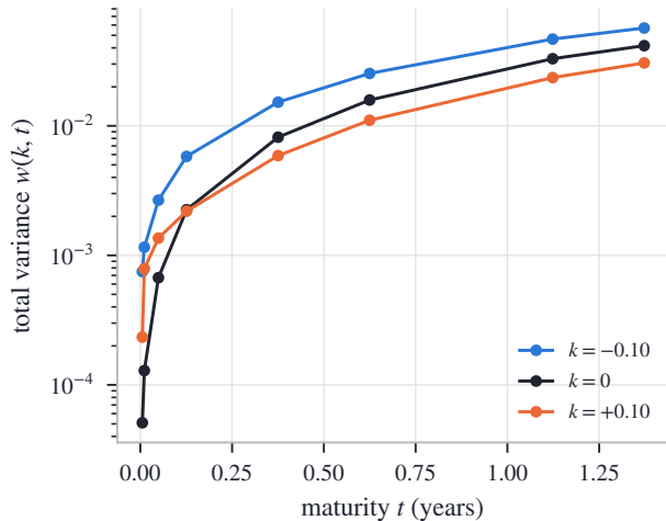
(a) convex order along the SPY strip
