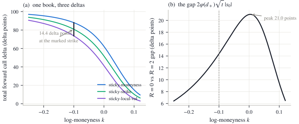
Figure 9.4: One book, three deltas (frozen hero node, eq. (9.4)). (a) Total forward call delta across strikes under the three regimes; at the marked k = -0.10 strike — a 19-delta put — the \mathcal{R} = 0 and \mathcal{R} = 2 answers are 14.4 delta points apart. (b) The gap (9.5) across strikes: a scaled vega profile, peaking at 21.0 delta points at the money.
