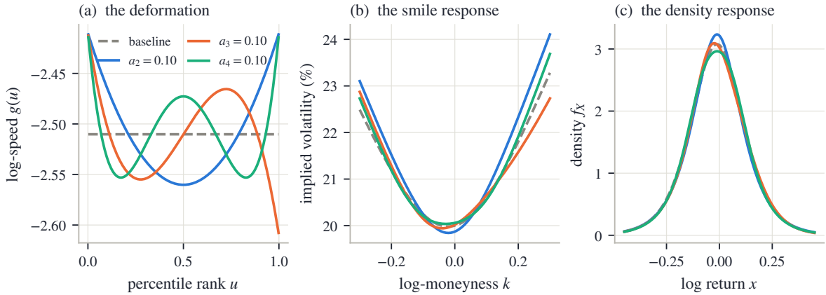
Figure 2.2: Three Legendre perturbations of the same reference law. Left: their action on log-speed g . Center: the response of implied volatility. Right: the response of the density. An even mode moves both endpoints in the same direction; an odd mode moves them in opposite directions. In all cases the density remains positive because the transport speed remains an exponential.
