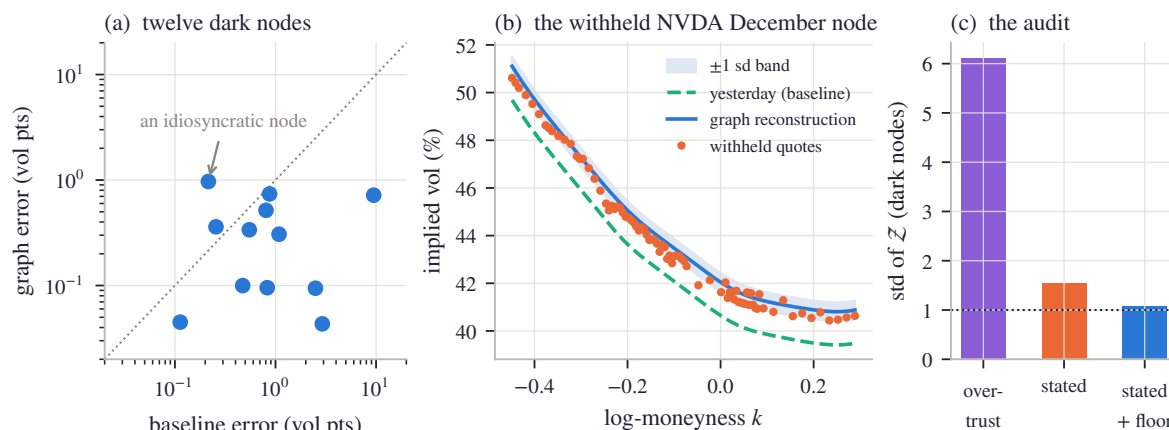
Figure 11.7: The universe completed. (a) Per-dark-node errors: graph against baseline, log-log; the diagonal is “no better than the prior.” 10 of twelve nodes sit below it; the nodes at or above it had idiosyncratic mornings, and the graph cannot know private moves. (b) The withheld NVDA December node: yesterday’s baseline (dashed), the graph’s retargeted reconstruction with its \pm 0.38 -point band (blue, shaded), and the frozen quotes the reconstruction never saw (orange). (c) The audit: std of the standardized dark-node errors — overtrusted precisions fail at 6.1; stated precisions read 1.55; adding the idiosyncratic floor lands 1.08, against the dotted target of one.
